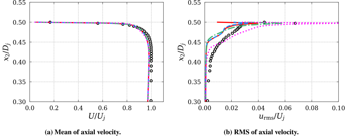
Fig. 8 Axial velocity statistics at the nozzle exit: Isolated-1 (—), Isolated-2 (---), Installed-1 (-.-.-), Installed-2 (.....), Experiments (○).
