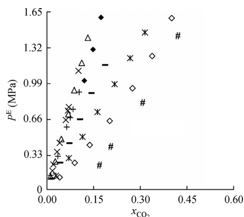
Fig. 6 CO 2 solubility in TTTM compared to that in ILs at 303.15 K. Symbols are: (♦) TTTM in this work; (#) [THTDP][NTf 2 ] (Carvalho et al., 2010); (×) [C 6 mim][BF 4 ] (Shokouhi et al., 2010); (—) [C 6 mim][OTf] (Jalili et al., 2010b); (+) [C 6 mim][PF 6 ] (Jalili et al., 2010b); (*) [C 8 mim][PF 6 ] (Safavi et al., 2013); (Δ) [C 2 mim][EtSO 4 ] (Jalili et al., 2010a), and (◇) [C 8 mim][NTf 2 ] (Jalili et al., 2012).
