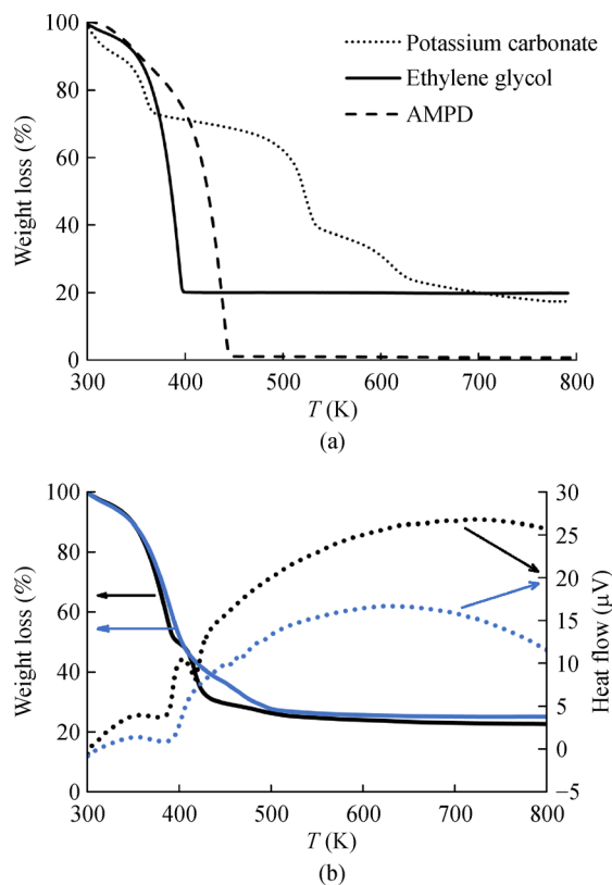
Fig. 3 (a) TGA curves for pure components and (b) TGA-DTA curves of prepared solvents from 300 K to 800 K at the heating rate of 10 K/min under Helium atmosphere with a flow rate of 100 mL/min. The black solid and dashed lines represent the TGA and DTA curves of TTM, respectively. The blue solid and dotted lines represent the TGA and DTA curves of TTTM, respectively.
