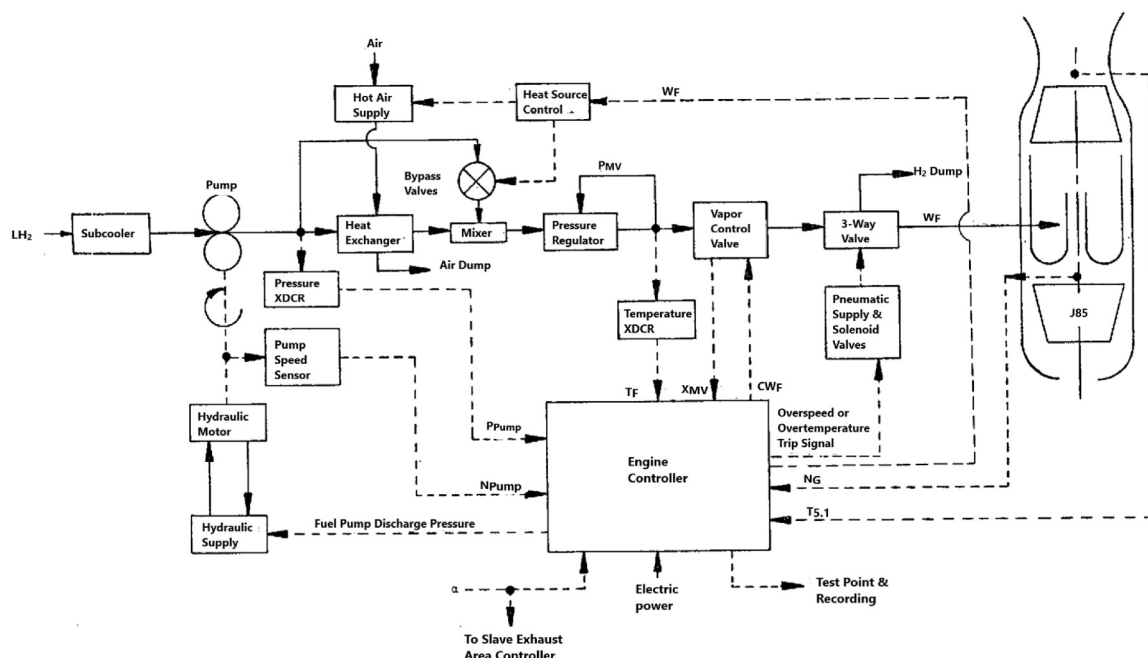
Fig. 8. J85 liquid hydrogen fuel system [35].
