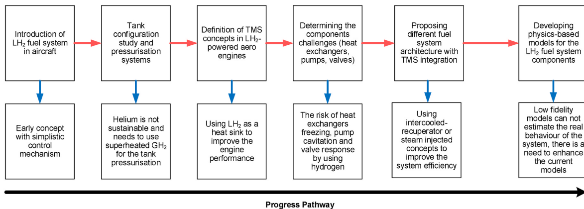
Fig. 19. Progression in liquid hydrogen fuel system concepts for aircraft engines.
