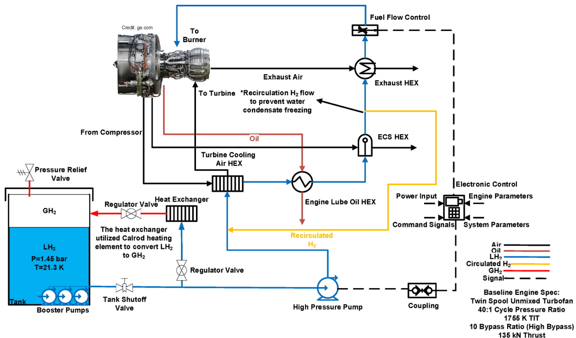
Fig. 9. NASA-Lockheed liquid hydrogen fuel system.
