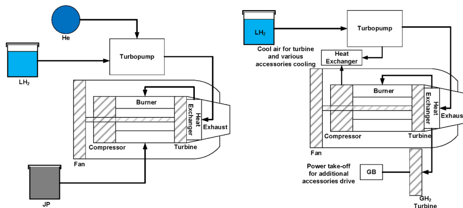
Fig. 13. Open-loop (left) and closed loop (right) systems, adapted from [47].
