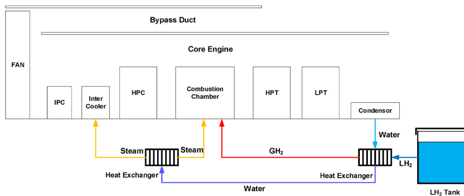
Fig. 17. Pratt &amp; Whitney HySiITE concept, adapted from [61].
