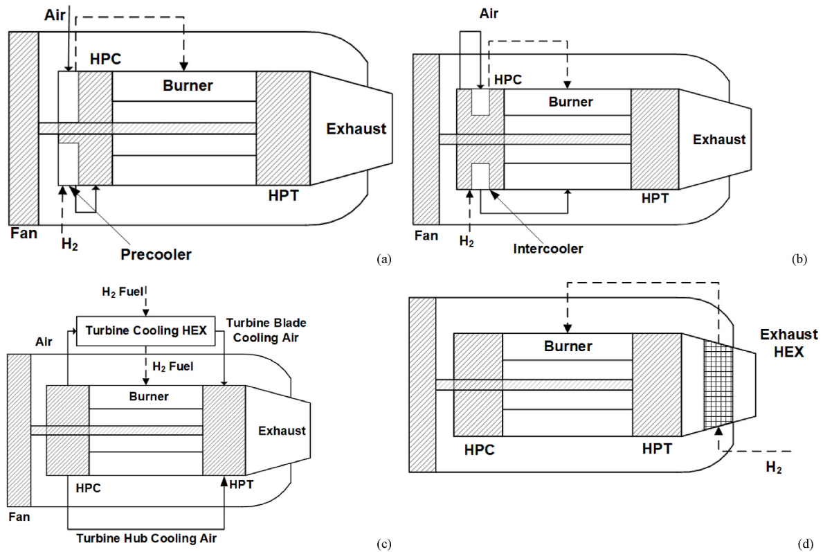
Fig. 10. Heat exchanger arrangements (a: precooler, b: intercooler, c: turbine cooling air, d: exhaust gas) - adapted from [39].
