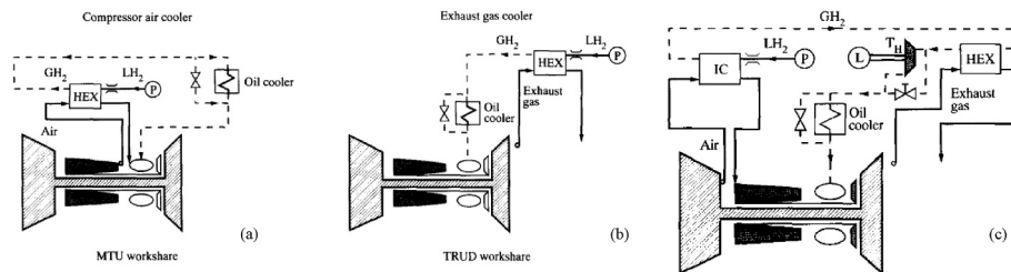
Fig. 11. Different fuel heater arrangements (a: compressor air cooler, b: exhaust gas cooler, c: integrated configuration) [46].
