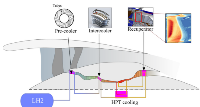
Fig. 14. Fuel heat management systems proposed in ENABLEH2 [42].
