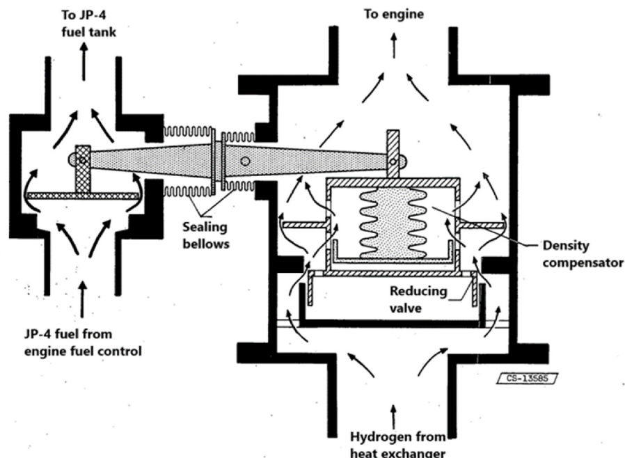
Fig. 6. B-57 JP-4 and hydrogen fuel ratio regulator [28].
