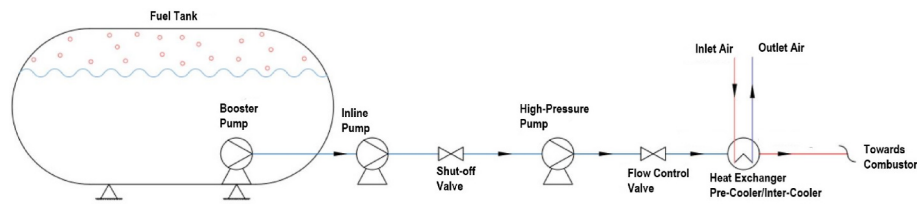
Fig. 15. Fuel distribution system proposed in ENABLEH2 [42].
