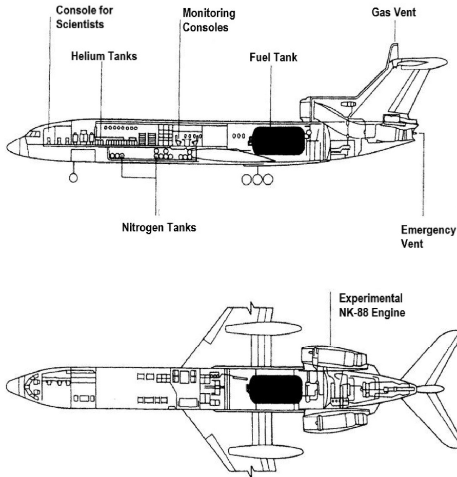
Fig. 12. Tu-155 aircraft configuration [48].
