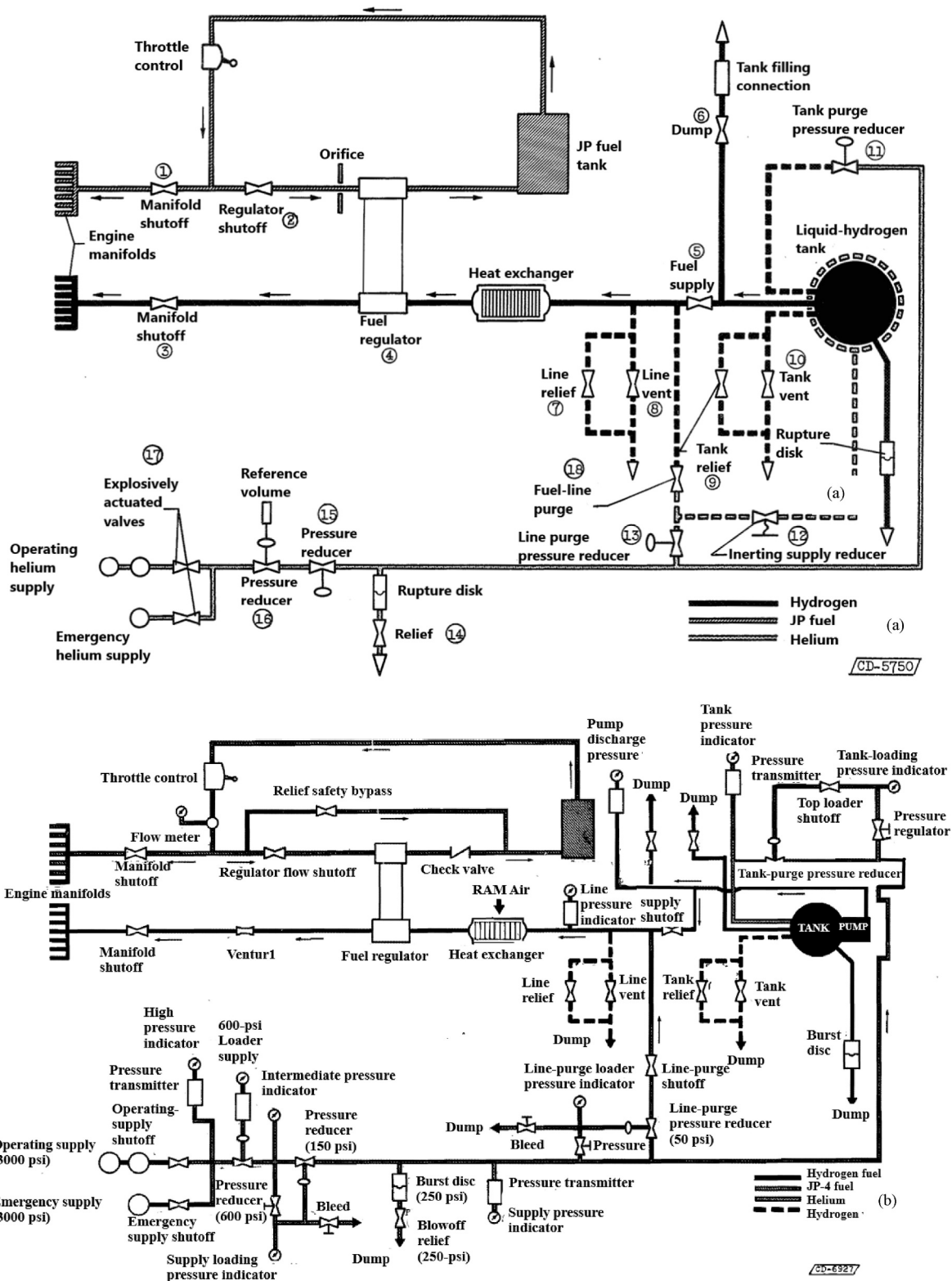
Fig. 7. B-57 liquid hydrogen fuel system schematic diagram (a: original with helium [33], b: modified with pump [34]).
