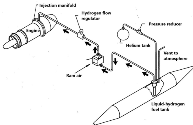
Fig. 5. B-57 hydrogen fuel system [28].
