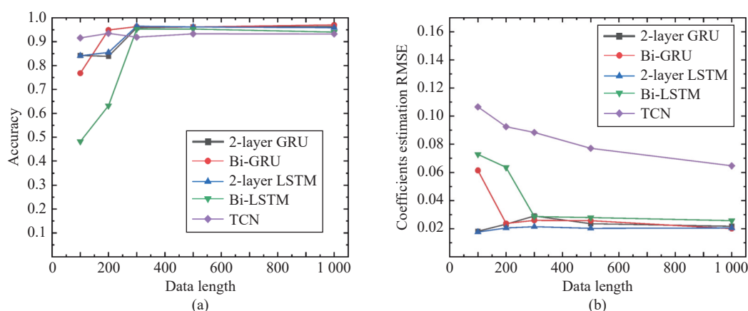
Fig. 6 The test results of different NN backbones with various data lengths. (a) Trend of the accuracy over the varying data length; (b) Trend of the RMSE of coefficients estimation over the varying data length. (Colored figures are available in the online version at https://link.springer.com/journal/11633 )
