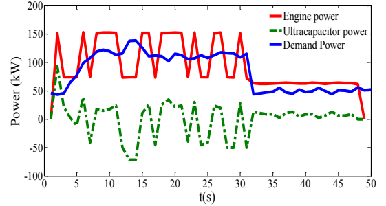
Fig.6 Dynamic programming results under scenarios 1
