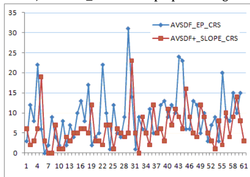
c) Two best combinations
