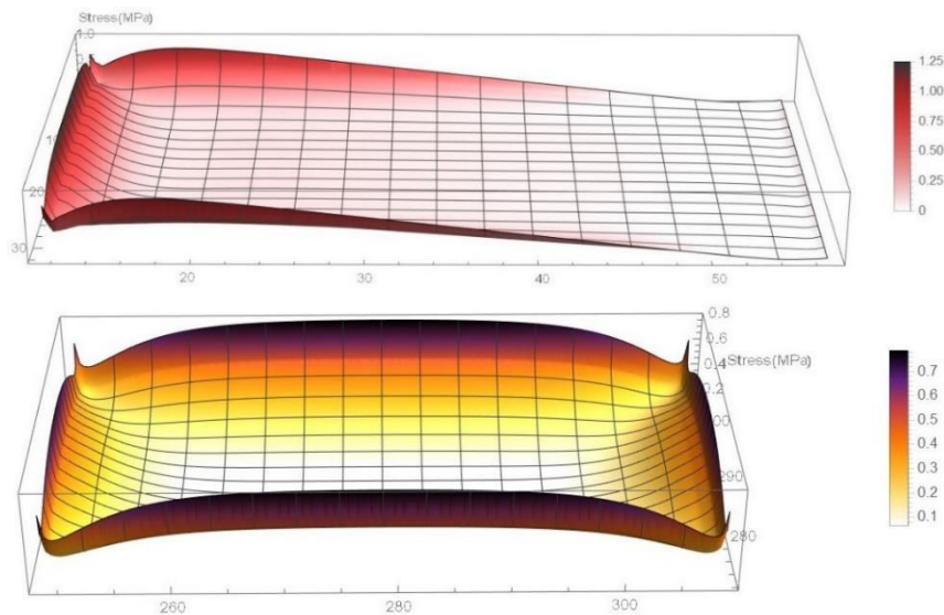
Figure 4: Normal Stress Distribution Across Short (Top) & Full (Bottom) Sample
