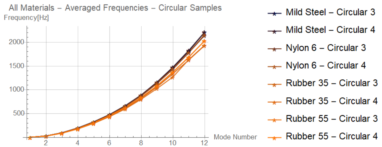
Figure 12: Bending Mode Distribution in Frequency Range
