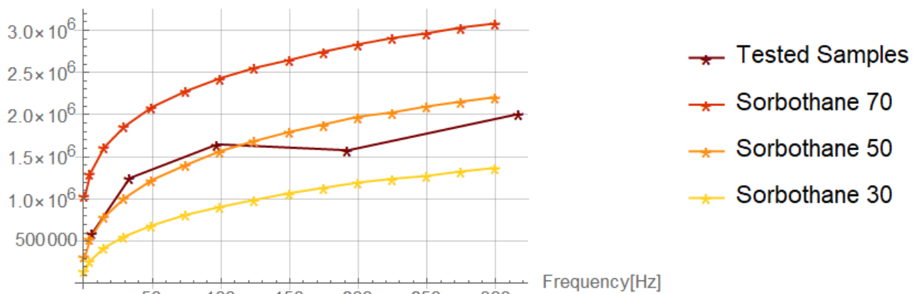
Figure 15: Sorbothane Dynamic Young's Modulus Characterisation & Comparison
