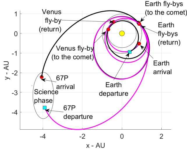
Fig. 22 Comet sample return trajectory to 67P involving an EVVE-67P trajectory to the comet (black path) and a 67P-EEVE transfer on the way back (magenta path).
