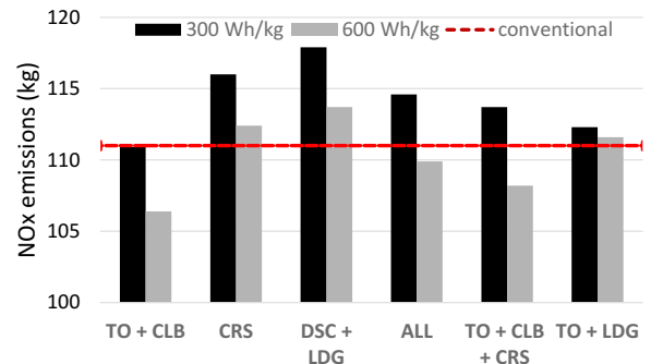
Figure 7: PMS influence on the NOx emissions for a 600 Wh/kg battery on a 450 nm mission
