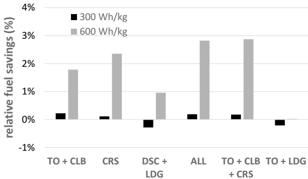
Figure 4: Fuel savings on a 450 nm mission
