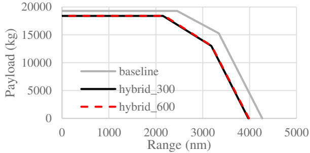
Figure 3: Payload range diagram comparison
