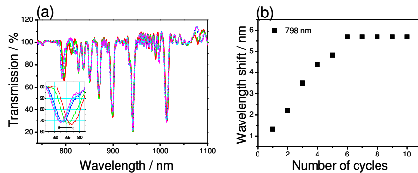
Fig. 7. (a) Changes in the transmission spectrum due to the alternate deposition of PDDA and SiO 2 NPs on the 400 \mu m period LPG, recorded in the colloidal SiO 2 solution; the inset shows an enlarged view of the resonance band at 798 nm. (b) Wavelength shifts at 798 nm.
