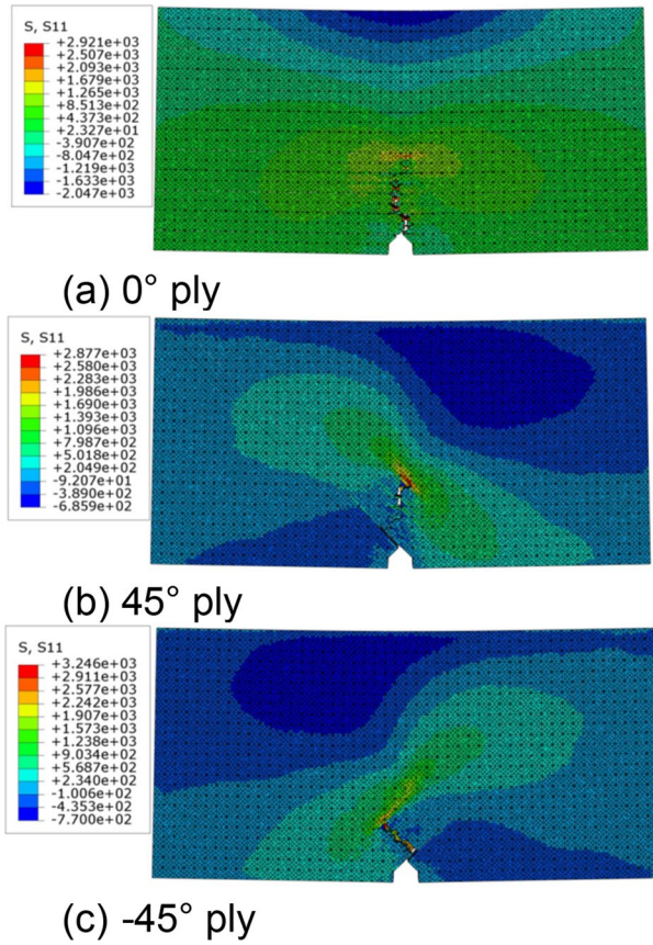
Fig. 5 Fibre direction stress distributions just after the peak load of 4.84 kN ( 100 \text{ kJ/m}^2 ) at room temperature dry conditions
