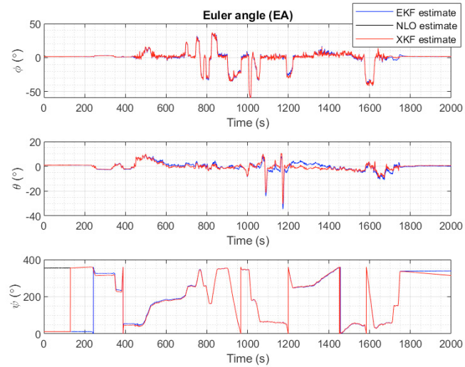
(a) Euler's angle estimation.
