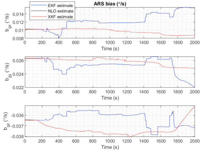
(b) Angular rate sensor's bias estimate.
