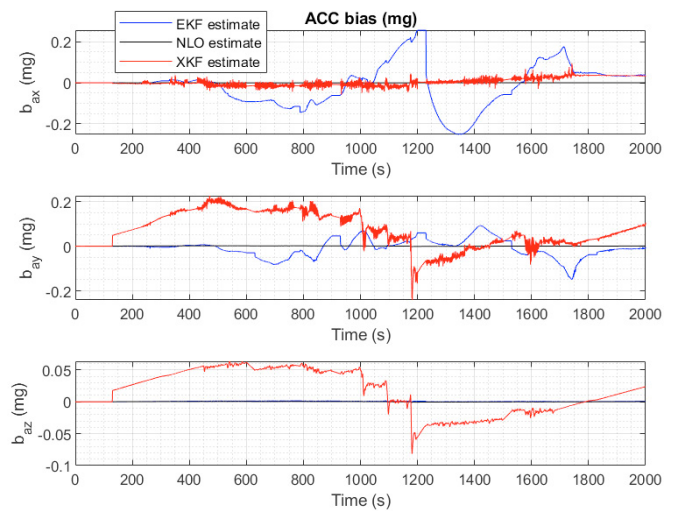
(e) Accelerometer bias estimation.
