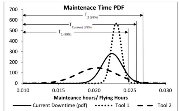
Figure 5: Comparison of maintenance time PDFs and their 99% confidence intervals.
