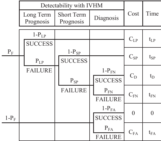
Figure 2: Event tree for the health monitoring of a single component and the possible outcomes of using different IVHM tools.
