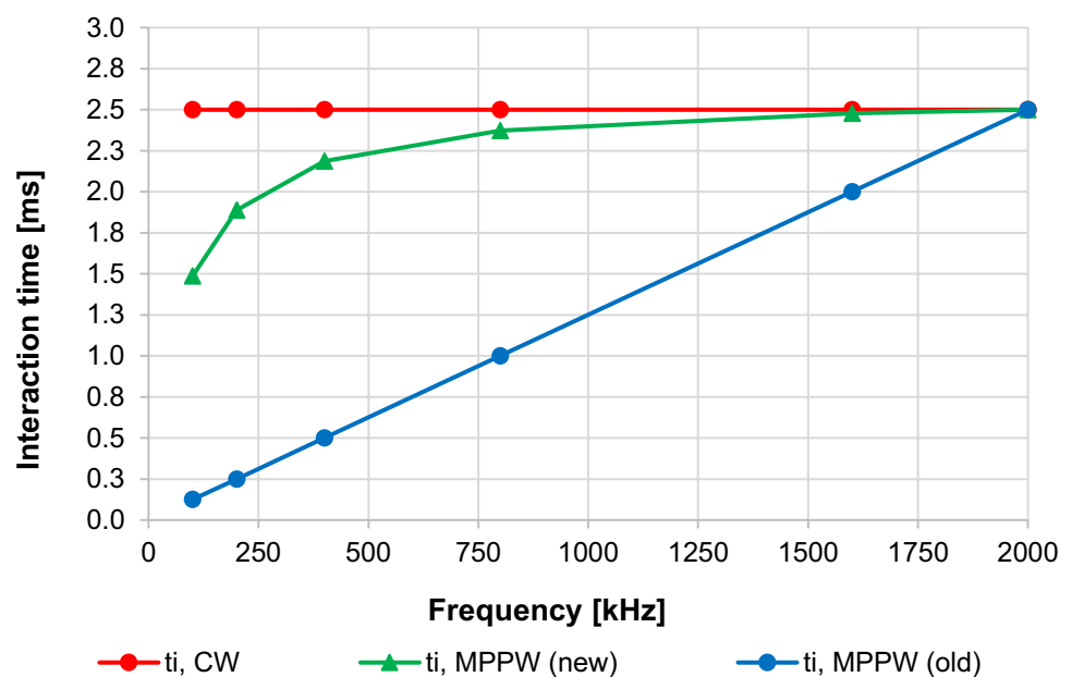
Fig. 7 Interaction times versus frequency for a constant travel speed of 56 mm/s, beam diameter of 35 \mu\text{m} and pulse width of 500 ns
