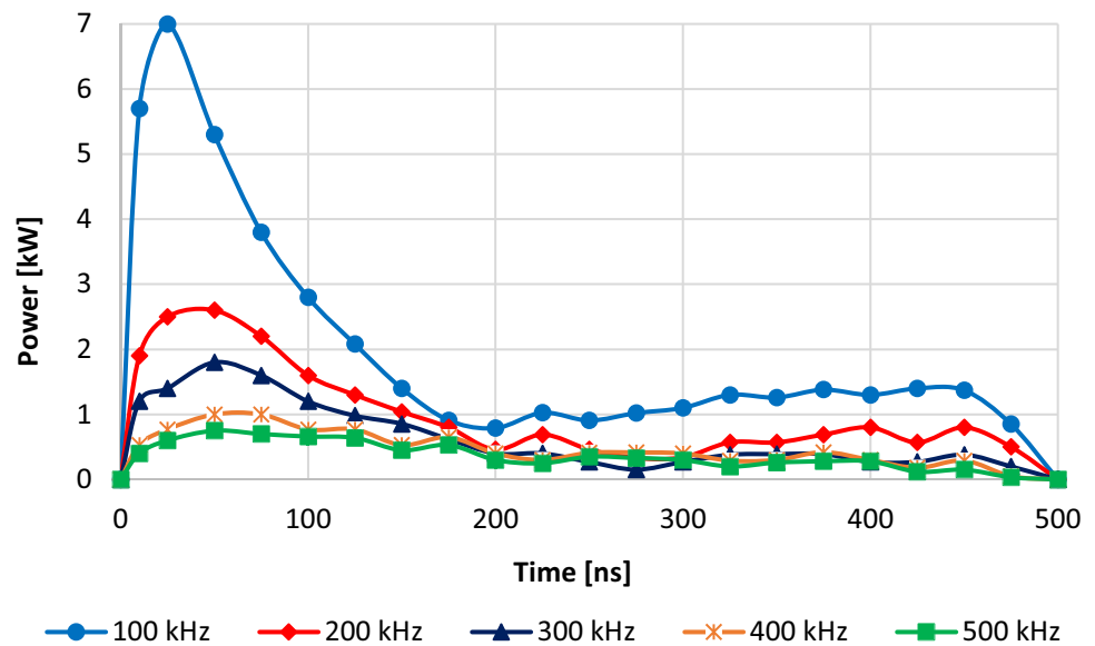
Fig. 3 Nanosecond MPPW laser temporal response for different pulse repetition frequencies at a constant average power of 100 W [25]
