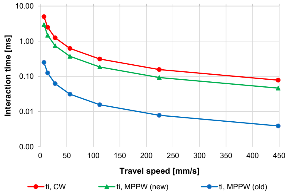
Fig. 6 Interaction times versus travel speed for a constant frequency of 100 kHz, beam diameter of 35 \mu\text{m} and pulse width of 500 ns
