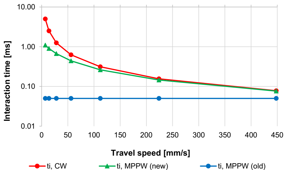
Fig. 5 Interaction times versus travel speed for a constant overlap factor of 99%, beam diameter of 35 \mu\text{m} and pulse width of 500 ns
