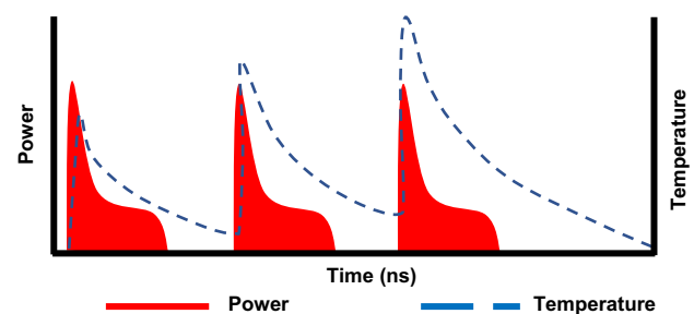
Fig. 4 Thermal cycle in nanosecond MPPW mode
