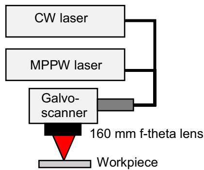
Fig. 8 Experimental setup of MPPW and CW fibre lasers used for stainless-steel welding
