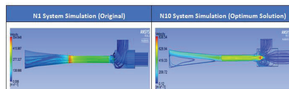
Figure 15: Ansys CFX simulation for system N1 and N10
