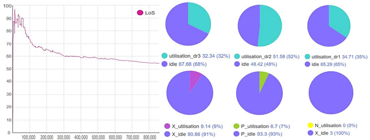
Figure 4: LOS and utilisation of resources.
