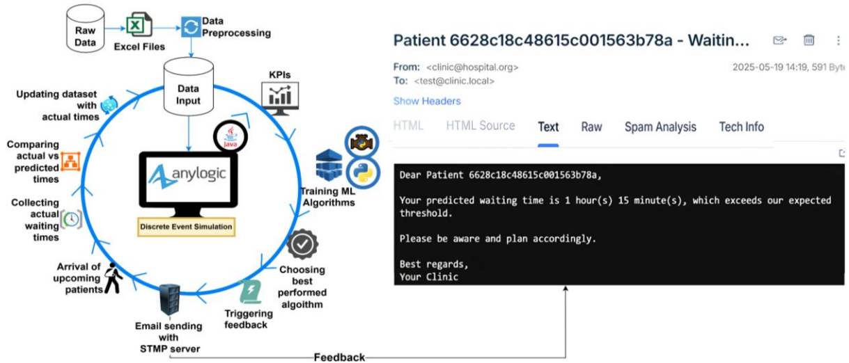
Figure 3: Workflow of the DT mechanism and dummy email snapshot.
