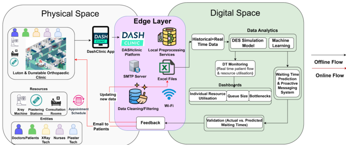
Figure 2: Digital twin conceptual architecture.
