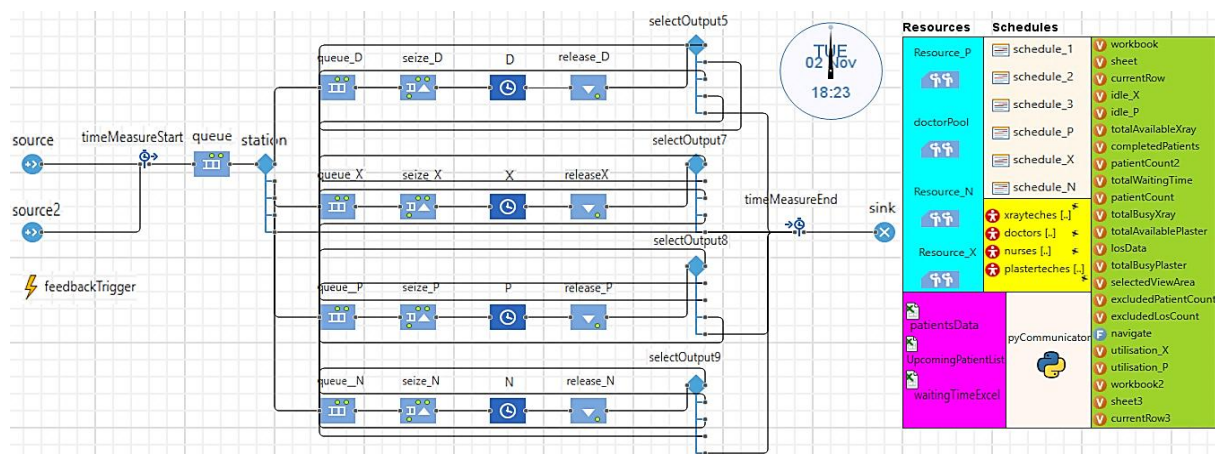
Figure 1: DES design of the clinic.
