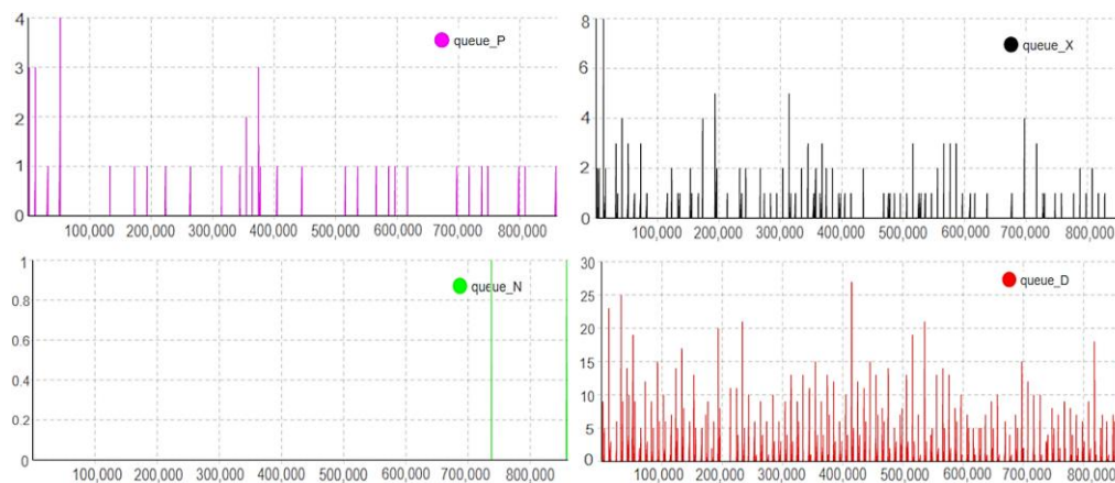
Figure 5: Queue size of the stations.
