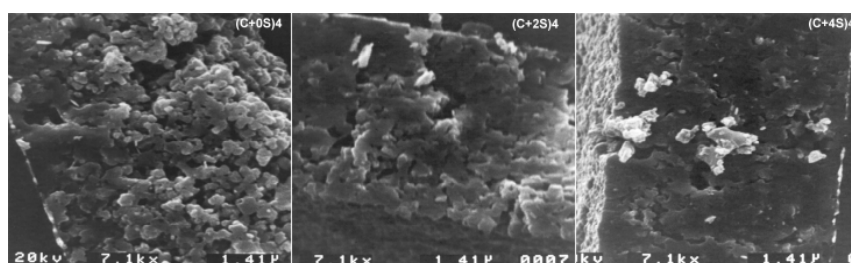
Figure 1 – SEM photomicrographs of fracture surfaces of films with different levels of sol infiltration/pyrolysis
