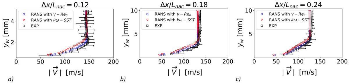
Fig. 8. Effect of turbulence model on boundary layer profiles at LDA measurements positions ( \Delta x/L_{nac} \approx 0.12, 0.18 and 0.24 ) on the nacelle cowl at mid-span ( \Delta z = 0 ); errorbars, plotted every 3rd point for figure readability, indicate the experimental uncertainty. h_{bump}/\Delta y_{rig,in} = 0.340 , M_{in} = 0.25 .
