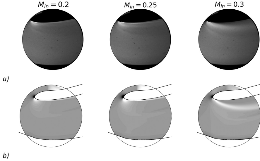
Fig. 14. Effect of inlet Mach number on the onset of nacelle boundary layer separation; (a) experimental schlieren photographs and (b) spanwise averaged density gradient ( \partial\rho/\partial y ) for the steady RANS with \gamma - Re_\theta turbulence model. h_{bump}/\Delta y_{rig,in} = 0.375 .
