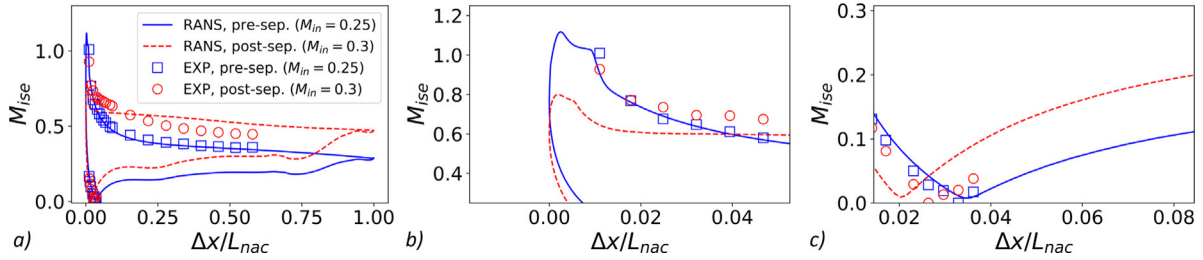
Fig. 15. Isentropic Mach number distribution on the nacelle cowl at mid-span ( \Delta z = 0 ) pre and post nacelle boundary layer separation; (b) and (c) zoom into peak M_{ise} and position of the stagnation point, respectively. h_{bump}/\Delta y_{rig,in} = 0.375 .
