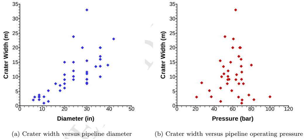
Figure 16: Crater width versus pipeline diameter and operating pressure individually.
