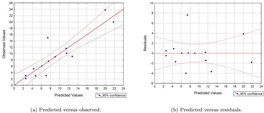
Figure 14: Accident-Based crater model scatterplots.
