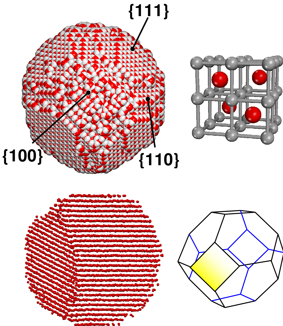
Figure 5 Final, low temperature, structure of the \text{Li}_2\text{O} nanocrystal (A) top left. Top right shows a segment cut from this nanocrystal revealing the inverse fluorite structure; bottom left shows a slice cut through the nanocrystal revealing the grain-boundary before it had annealed out of the structure during prolonged MD; bottom right a schematic illustrating the truncated octahedral morphology. Lithium is coloured grey and oxygen is red.
