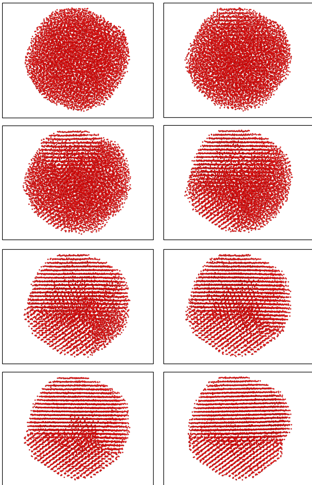
Figure 3 Snapshots of the atom positions comprising the \text{Li}_2\text{O} nanoparticle (A), taken during the molecular dynamics simulation, revealing the evolution of a crystalline nanoparticle from an amorphous precursor; only the oxygen ions (red) are shown to improve clarity.
