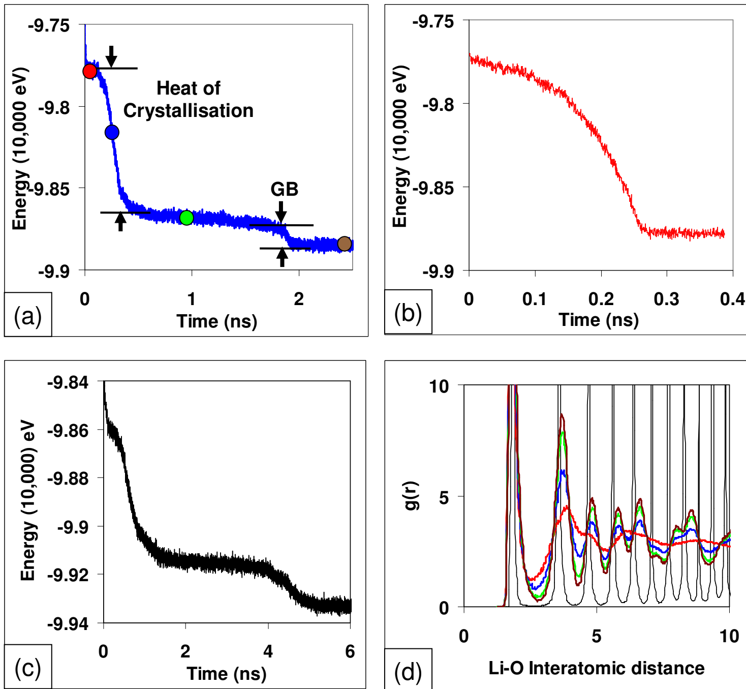
Figure 1 Configuration energy, calculated as a function of time, during crystallisation. (a) \text{Li}_2\text{O} nanoparticle (A). (b) \text{Li}_2\text{O} nanoparticle (B); (c) \text{Li}_2\text{O} nanoparticle (C). (d) Radial Distribution Function (RDF) for \text{Li}_2\text{O} nanoparticle (A), calculated after: 130 ps (red); 260 ps (blue); 1000 ps (green); 2000 ps (brown) and for the final, 0K structure (black). The RDF can be usefully correlated with figure 1(a), on which are shown coloured circles corresponding to the RDF.
