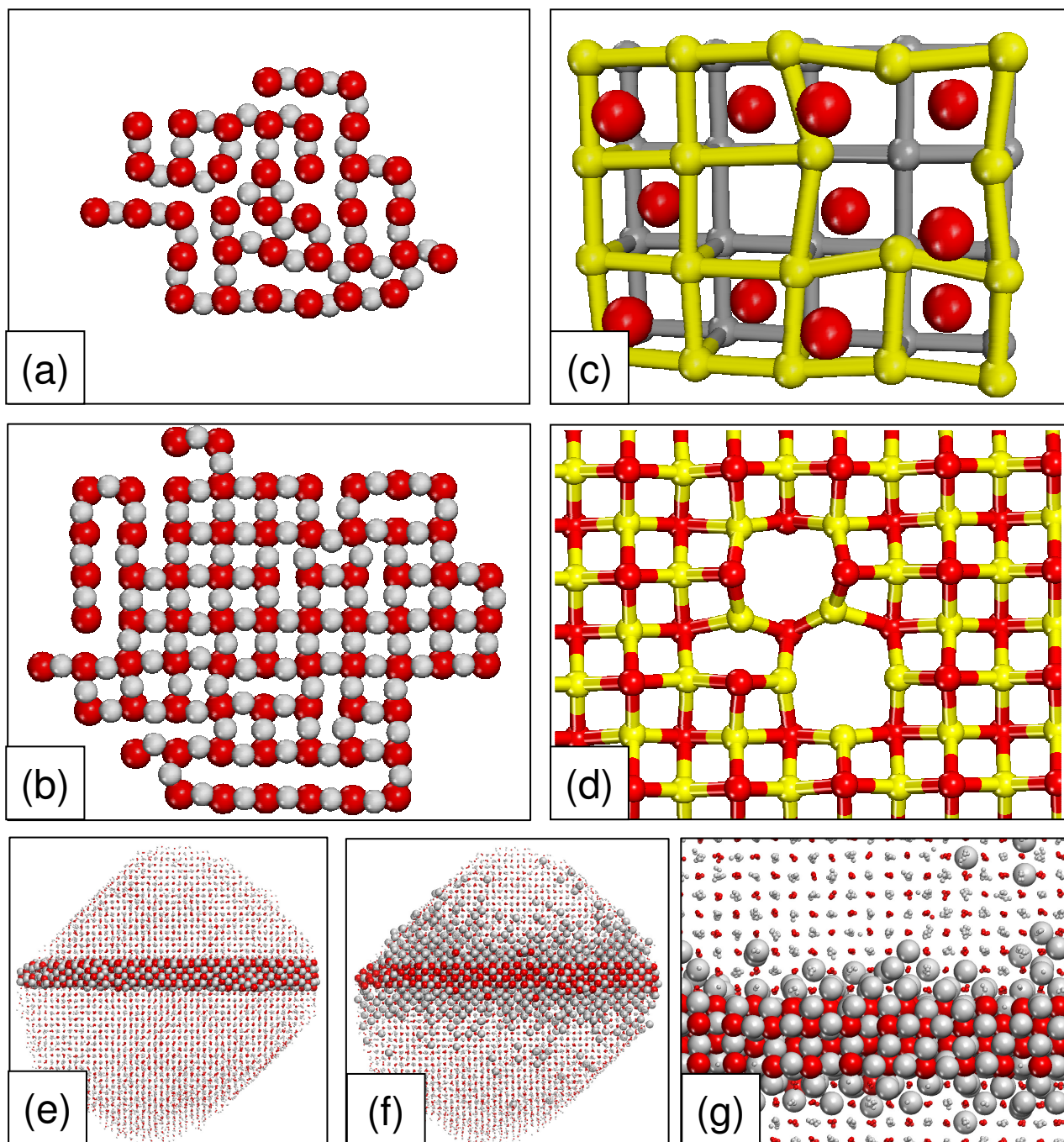
Figure 7 Structure of the surface atomic layer (a) and penultimate surface atomic layer (b) of the (dipolar) (100) surface revealing how the dipole is quenched via a 50% reduction of Li ions at the surface to give LiO stoichiometry; (c) and (d) reveal the structure of point defects that have evolved within the \text{Li}_2\text{O} nanocrystals; (e) \text{Li}_2\text{O} nanocrystal (C) after 9 ns of MD and (f) after 19 ns of MD simulation revealing the mobility of the Li ions; (g) enlarged segment of (f). Oxygen is coloured red and Li is grey or yellow.
