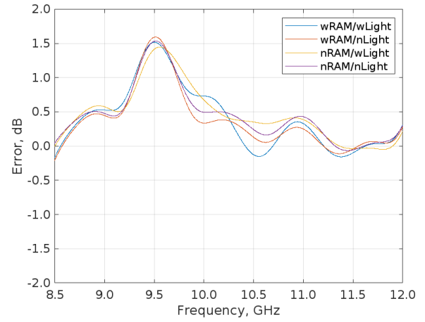
Fig. 7. Calibration error in \text{dBm}^2 of the 38 mm sphere calibrated against the 80 mm sphere.
