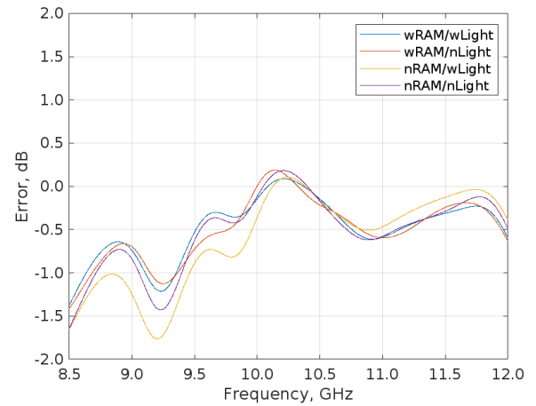
Fig. 9. Calibration error in \text{dBm}^2 of the 80 mm sphere calibrated against the 30 mm sphere.
