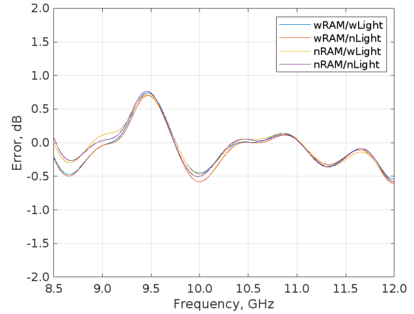
Fig. 14. Calibration error in \text{dBm}^2 of 100 mm sphere calibrated against 80 mm sphere.
