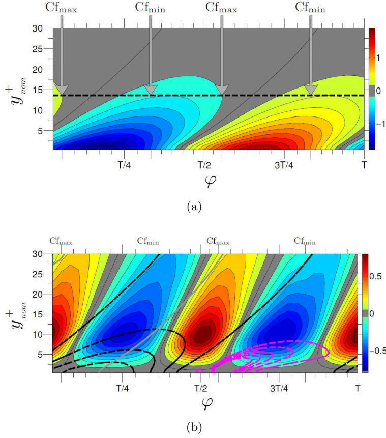
Figure 26: Contours of spanwise strain rate as function of phase during the actuation cycle (top) and corresponding contours of phase-averaged streamwise stress relative to time-averaged field (bottom) at Re_\tau = 1000 , T^+ = 200 ; black curved dashed lines indicate spanwise strain; gray curved lines are loci of maximum Stokes strain; magenta lines indicate skewness \partial\theta/\partial y . Reproduced from Agostini et al. [2014], with permission from CUP.
