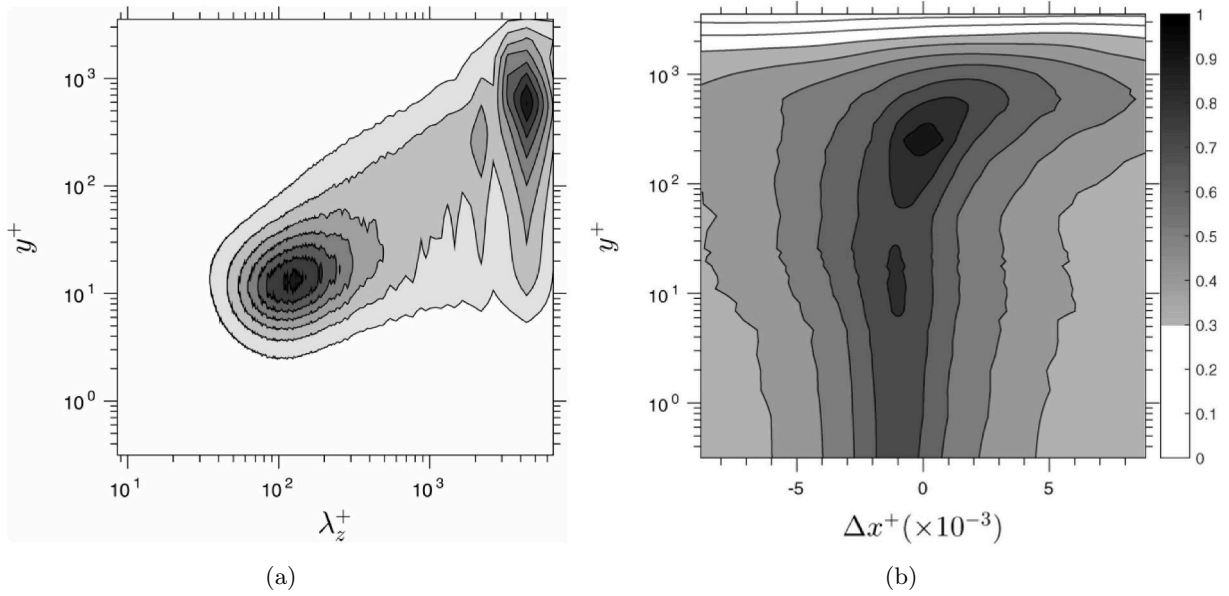
Figure 38: Manifestations of large-scale outer structures in channel flow at Re_\tau = 4200 (DNS by Lozano-Durán and Jiménez [2014b]); (a) spectral map of streamwise energy in wall-normal-distance/spanwise-wavelength plane: peak of large-scale energy at y^+ \approx 400 , \lambda_z^+ \approx 4000 ; (b) map of two-point correlation of large-scale fluctuations relative to location y^+ = 250 . Taken from Agostini and Leschziner [2016], with permission from AIP Publishing.
