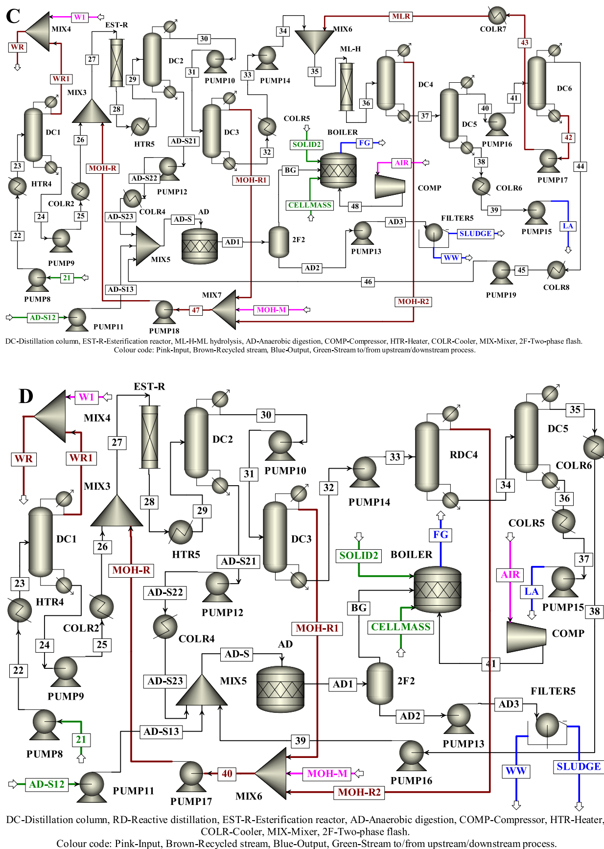
Figure 1. Process flowsheet for the fermentative production of LA from SCB without process integration using (A) alkali pretreatment and (B) acid pretreatment. Downstream separation of LA (C) by CD and (D) RD for alkali pretreatment.
