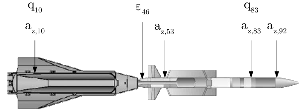
Figure 2: Output selection: strain gauges \varepsilon , gyroscopes q and accelerometers a_z ; missile length is 4.9 \text{ m} and there are n = 100 uniformly-spaced nodes as candidate locations for sensor placement
