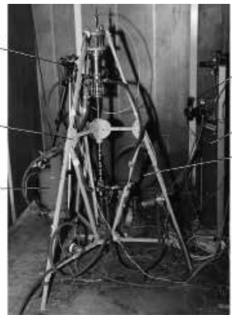
Fig. 9 The experimental rig in the rocket motor test cell. Key: (a) layout of the main equipment; (b) overview showing 1. the experimental rig; 2. the video camera; 3. the carbon dioxide cylinder; 4. the propane bottle; 5. the extractor of combustion products; 6. the oxygen cylinder; 7. the nitrogen cylinder; 8. the walls, roof and door; 9. the electric power supply; 10. the high voltage coil; 11. the high voltage wires; 12. the control panel; 13. the temperature sensor line; 14. the pressure sensor line; 15. the data logger and 16. the nitrous oxide bottle.
