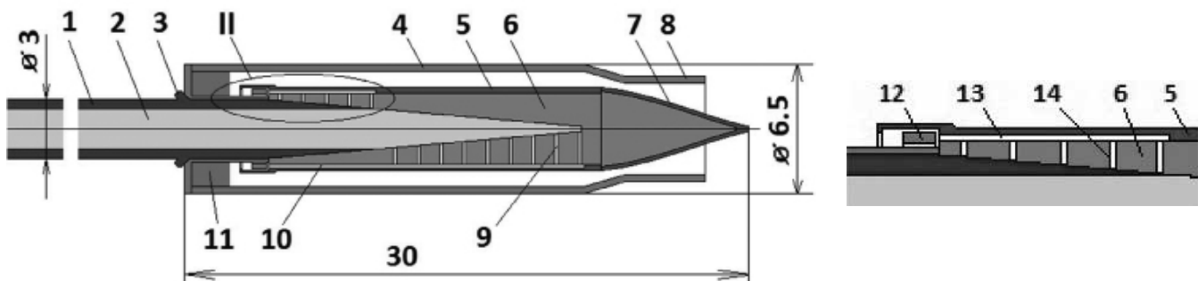
Fig. 15 Propellant cartridge of a self-feeding micropropulsion unit. Dimensions are in millimetres. Key: 1. polymeric fuel; 2. solid oxidizer; 3. seal – a collar of melted fuel; 4. the combustion chamber case; 5. the gasification chamber steel case; 6. the gasification chamber of copper; 7. thermal coating; 8. the nozzle; 9. an oxidizer hole; 10. the oxidizer duct; 11. the space for a solid propellant igniter; 12. the ring valve; 13. the fuel duct and 14. a fuel hole.
