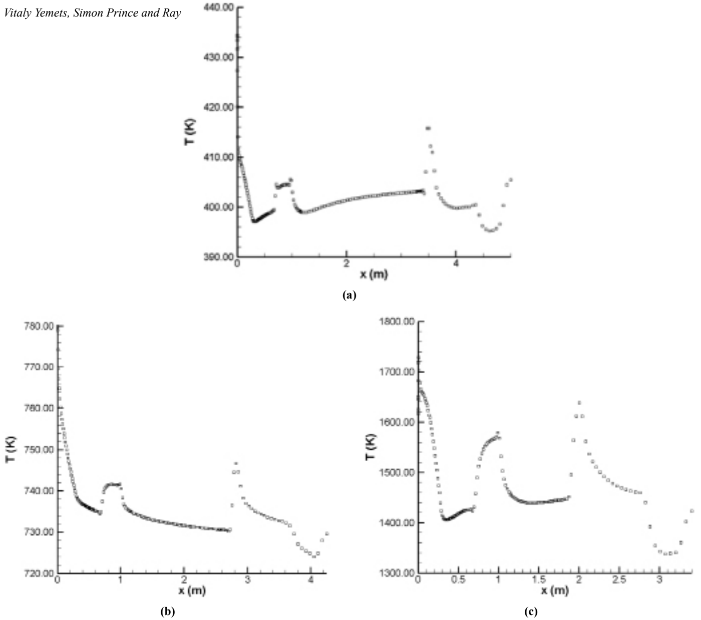
Fig. 2 The temperature of the contracting rocket airframe surface at the following instants of time following the rocket launch: (a) 5.5 s, (b) 10 s, (c) 14 s.
