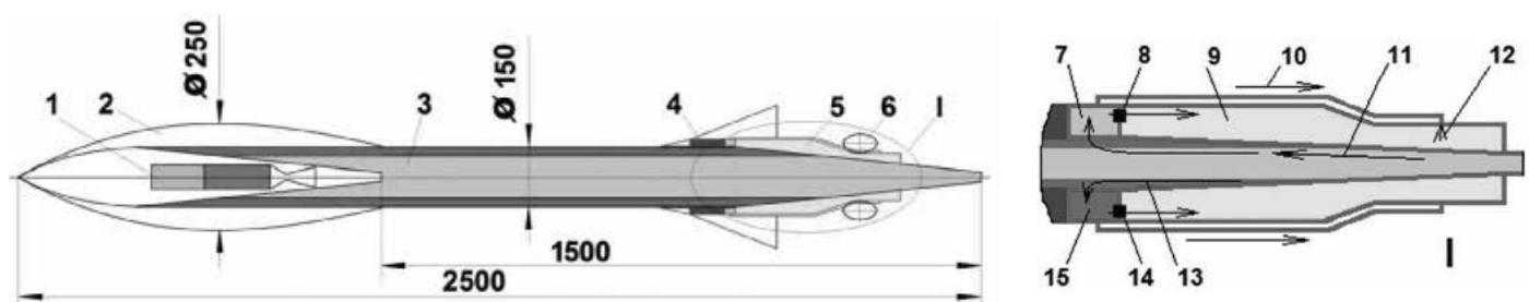
Fig. 13 A small combustible pulse LV concept with an initial mass of about 50 kg capable of orbiting a 100 g payload into a low orbit. Dimensions are in millimetres. Key: 1. the payload attached 2 nd solid stage; 2. a variable geometry inflatable nose fairing; 3. the combustibile case of polymeric pipe filled with solid oxidizer; 4. an obturator; 5. the mobile engine; 6. a restart system; 7. the oxidizer chamber; 8. the oxidizer valve; 9. the combustion chamber; 10. gasiform propellant component flow to control injector; 11. gasiform oxidizer flow; 12. a control injector; 13. gasiform fuel flow; 14. the fuel valve and 15. the fuel chamber.
