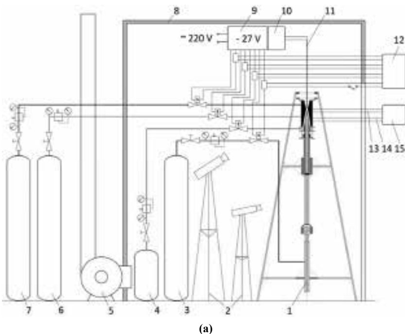
Fig. 9 The experimental rig in the rocket motor test cell. Key: (a) layout of the main equipment; (b) overview showing 1. the experimental rig; 2. the video camera; 3. the carbon dioxide cylinder; 4. the propane bottle; 5. the extractor of combustion products; 6. the oxygen cylinder; 7. the nitrogen cylinder; 8. the walls, roof and door; 9. the electric power supply; 10. the high voltage coil; 11. the high voltage wires; 12. the control panel; 13. the temperature sensor line; 14. the pressure sensor line; 15. the data logger and 16. the nitrous oxide bottle.
