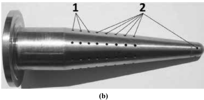
Fig. 8 The gasification chamber. Key: (a) drawing dimensioned in millimetres; (b) overview; 1. fuel holes; 2. oxidizer holes.
