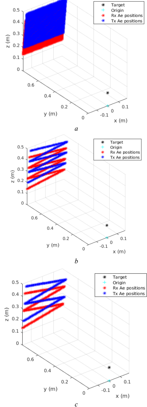
Fig. 7 Scanned transmitter and receiver horn positions and scene geometry:
