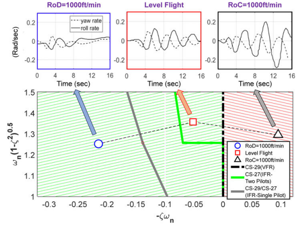
Figure 13: Flight test results from RAE research Puma (SA330) showing variations of LDO stability, and roll/yaw responses to pedal doublet, with vertical flight path, 100kts airspeed (Refs. 21, 22)
