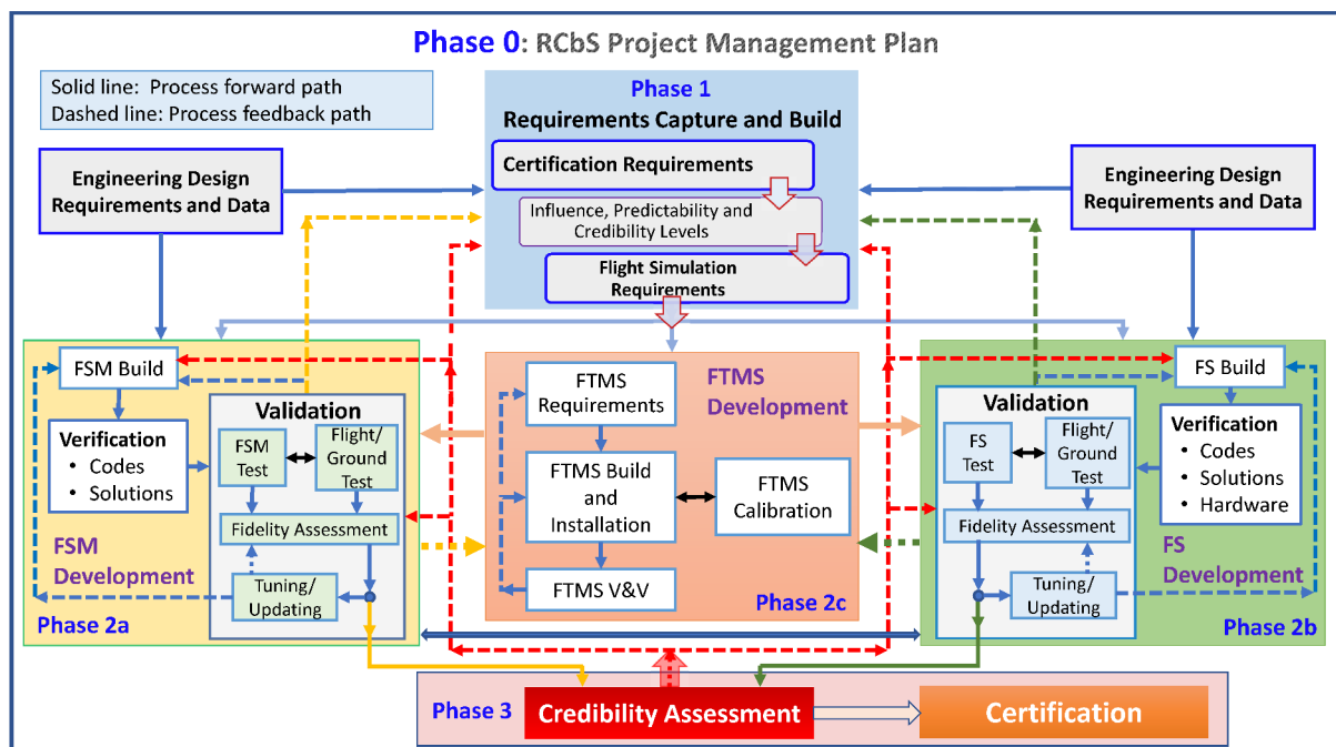
Figure 1: The RCbS process summarised (Refs 9, 10)
