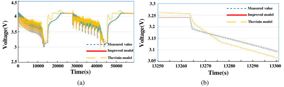
Fig. 11 Comparison of model verification results under DST-UDDS: (a) Full test; (b) Partial enlargement.
