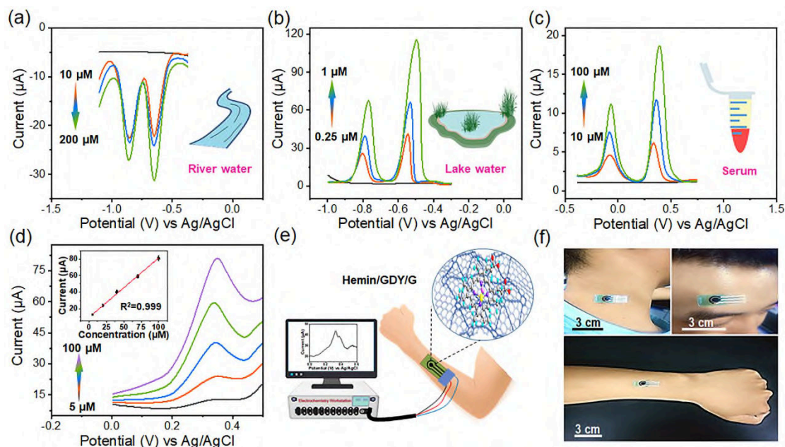
Fig. 5. (a, b) The real sample analysis of GDY/G/GCE. (a) River water with different amounts of NB and 4-NP in pH 7.0. (b) Lake water with different amounts of \text{Cd}^{2+} and \text{Pb}^{2+} in pH 5.0. (c) The real sample analysis of hemin/GDY/G/GCE in serum with different amounts of AA and UA in pH 7.0. (d) DPV curves of different UA (5, 20, 40, 70, and 100 \mu\text{M} ) concentrations at hemin/GDY/G modified screen-printed electrode. Inset shows the linear relationship between peak current and UA concentration. (e) Schematic diagram of the flexible and wearable sensor for UA sensing in human sweat. (f) Demonstration photos of the wearable biosensors attached on different parts of the body for monitoring.
