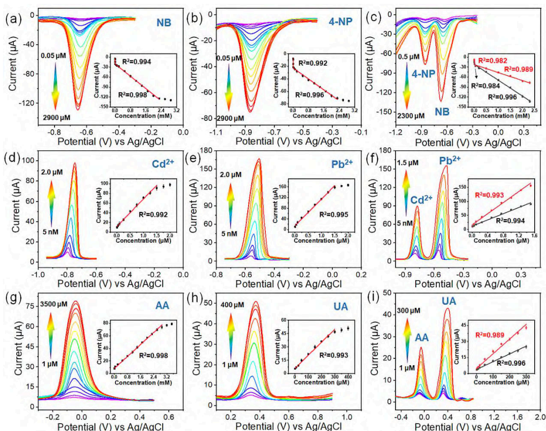
Fig. 3. (a~c) DPV curves of the GDY/G/GCE towards the detection of (a) NB, (b) 4-NP, (c) NB and 4-NP. (d~f) DPASV curves of the GDY/G/GCE towards the detection of (d) Cd^{2+} , (e) Pb^{2+} , (f) Cd^{2+} and Pb^{2+} . (g~i) DPV curves of the hemin/GDY/G/GCE towards the detection of (a) AA, (b) UA, (c) AA and UA. Inset shows linear trend of the peak current versus concentration of corresponding analytes.
