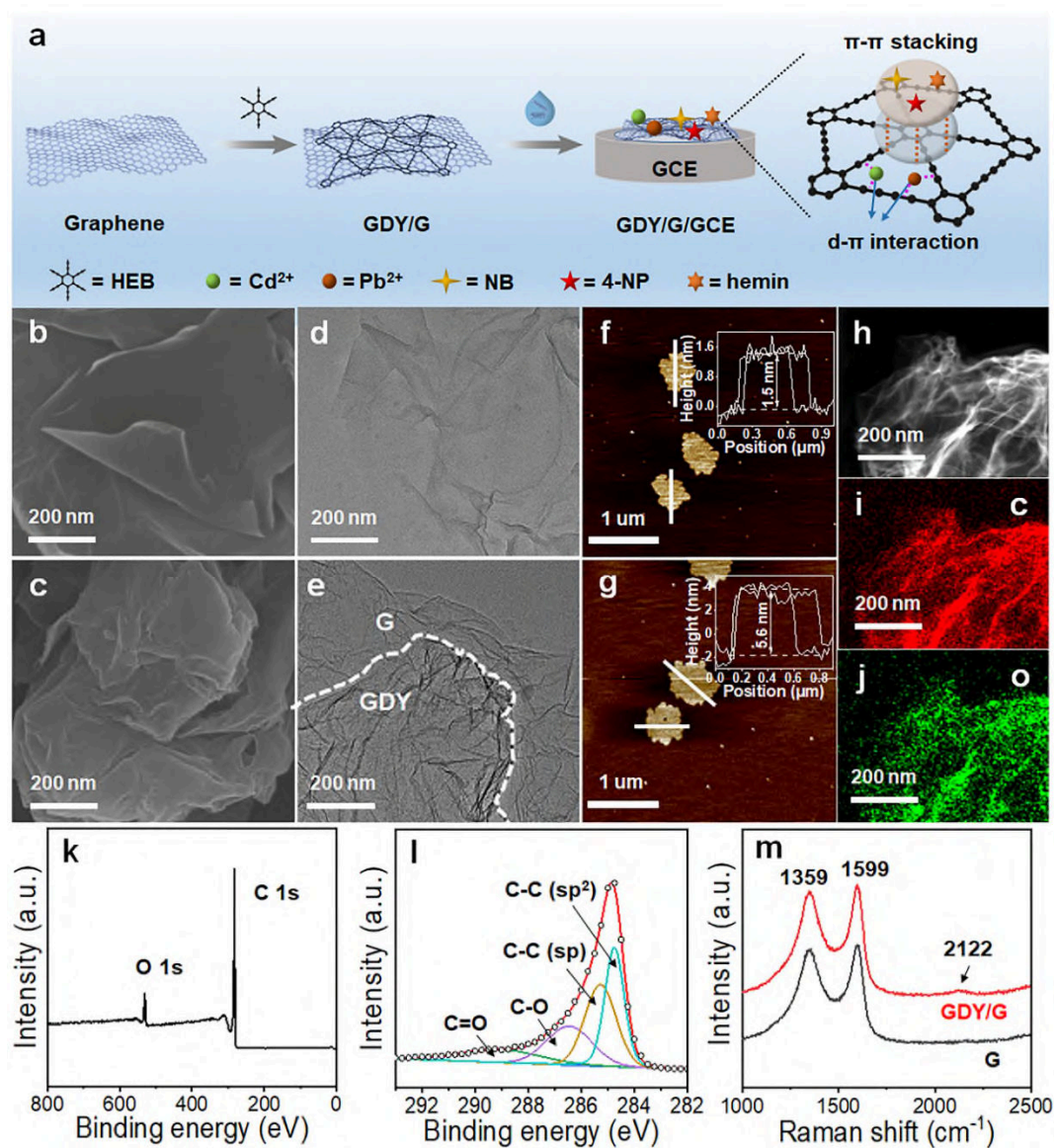
Fig. 1. (a) Schematic illustration of the preparation of GDY/G heterostructure and its application in the detection of heavy metal ions ( \text{Cd}^{2+} , \text{Pb}^{2+} ) and toxic molecules (NB, 4-NP). (b~g) SEM, TEM, and AFM images of (b, d, f) graphene and (c, e, g) GDY/G. (h~j) STEM image and EDS elemental maps of GDY/G for (i) C and (j) O elements. (k) XPS survey spectra of GDY/G. (l) XPS C 1s spectrum of GDY/G. (m) Raman shift of graphene and GDY/G.
