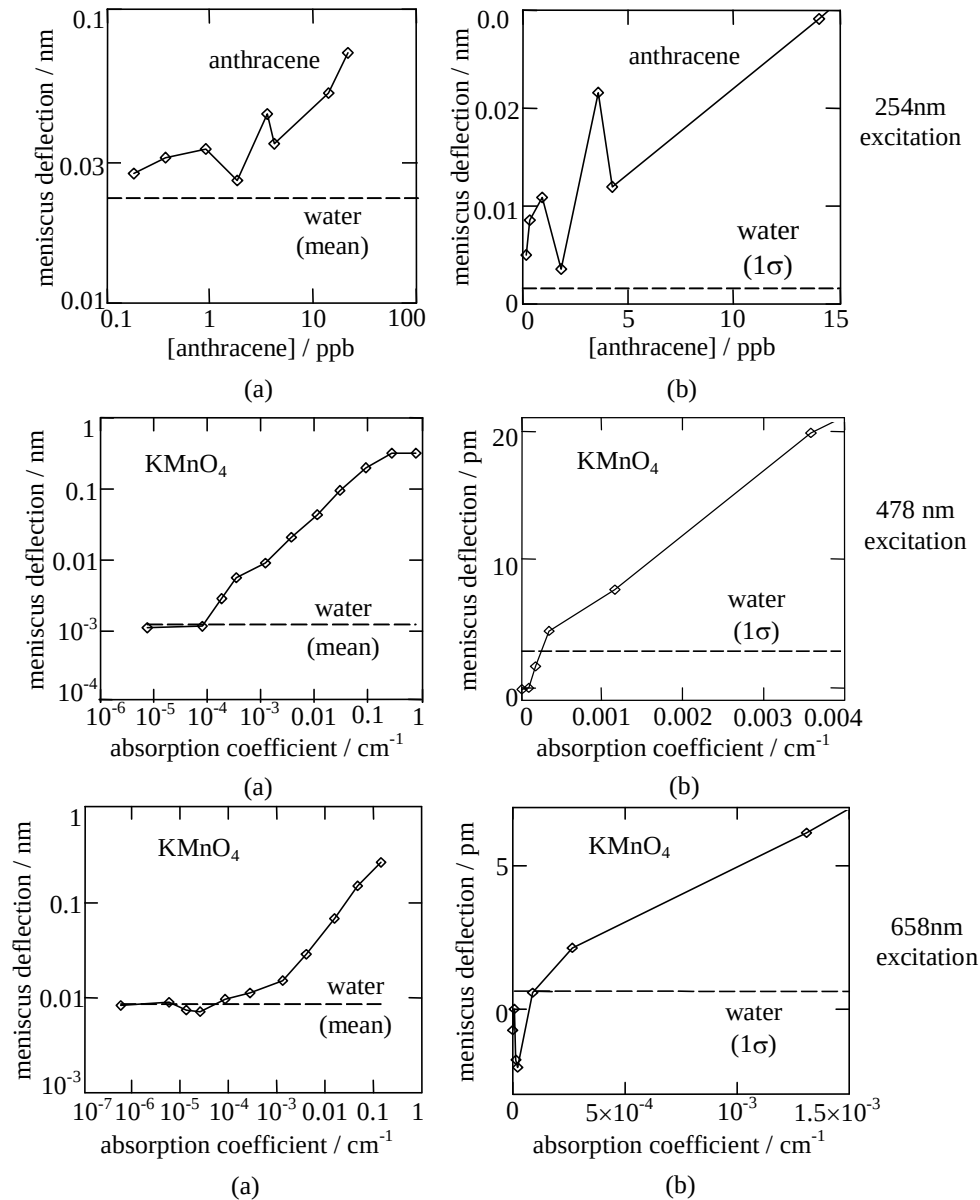
Figure 6. Photothermal rms meniscus deflection excited in \text{KMnO}_4 solutions by a 478nm and 658nm LED (as previously published [4] ) and in anthracene solutions by a mercury discharge lamp. (a) Original data. (b) The same data following subtraction of the mean measurement for water.
