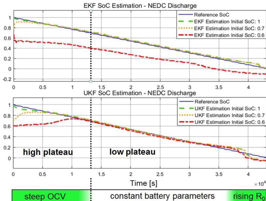
Figure 1. The Extended Kalman Filter (EKF) and Unscented Kalman Filter (UKF) have been demonstrated for use on real lithium-sulfur cells subject to automotive drive cycles: the UKF was found to cope better with unknown initial states of charge. 8
