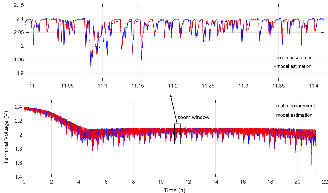
Figure 7. Li-S cell terminal voltage prediction vs. real measurement.
