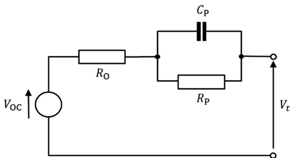
Figure 3. Thevenin battery model.
