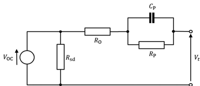
Figure 9. Thevenin battery model with self-discharge resistance.
