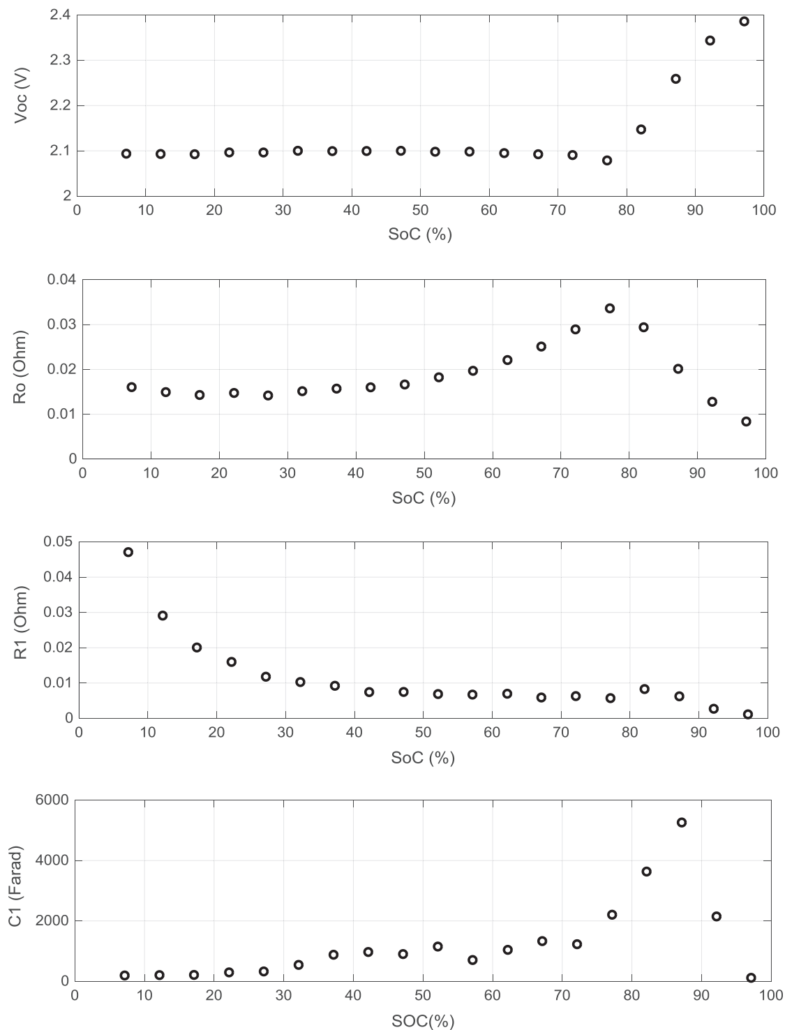
Figure 6. Thevenin model parameterization for a 21 Ah Li-S cell: the four unknown parameters are obtained as a function of SoC.
