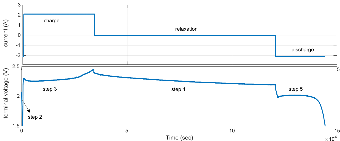
Figure 10. Systematic self-discharge experiment steps.
