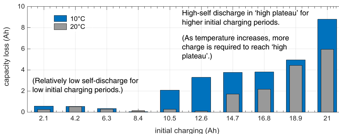
Figure 11. Capacity loss of a 21 Ah Li-S cell due to self-discharge during 24 hours.
