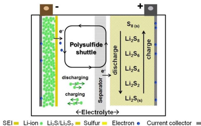
Figure 8. Schematic of polysulfide shuttle in a Li-S cell.
