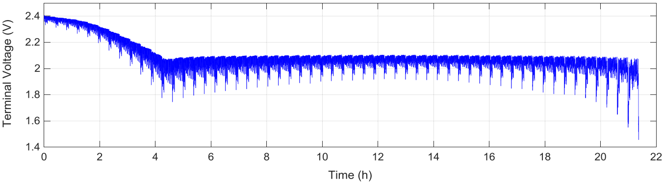
Figure 5. Terminal voltage of Li-S cell subjected to UDDS current profile.
