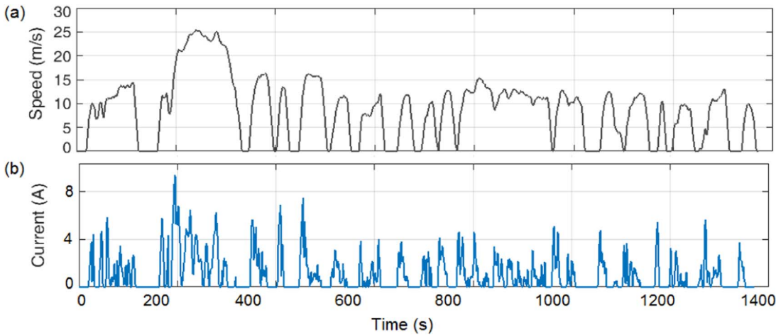
Figure 4. UDDS velocity profile and the scaled current profile.
