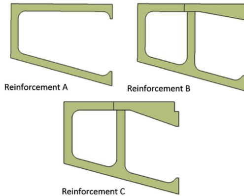
Fig. 5. Structural reinforcements of the floater.
