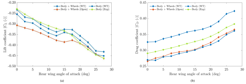
Figure 8: (a) Lift coefficients and (b) drag coefficients results from the experiments (Exp), 'wind tunnel' simulations (WT), and 'open road' simulations (Open)
