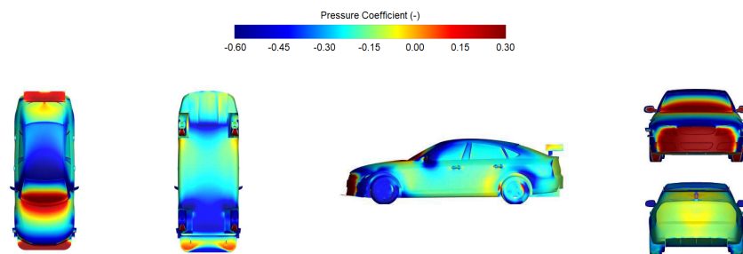
Figure 12: Pressure coefficient distribution on the vehicle in straight-line conditions with a 0^\circ rear wing angle of attack
