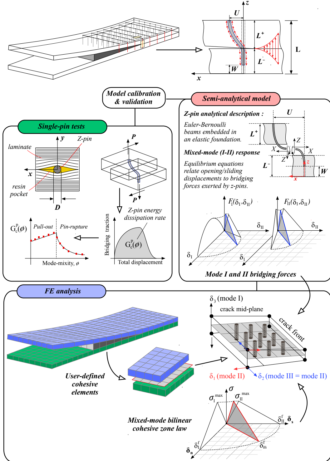
Figure 2: Multi-scale modelling philosophy for through thickness reinforcement
