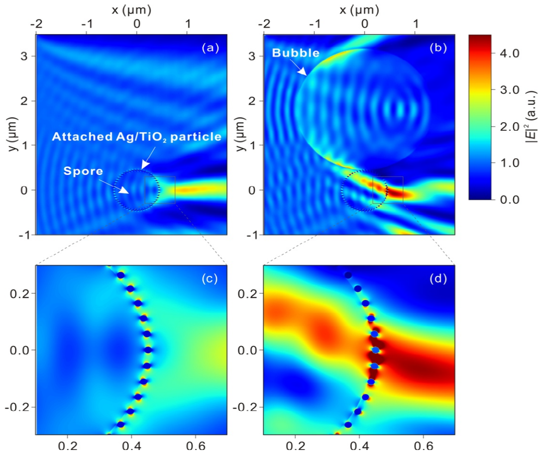
Fig. 6. (a) Electric field distribution near an illuminated spore with attached Ag/TiO 2 particles. The incident wavelength is 500 nm. (b) Electric field distribution near an illuminated MNB with a nearby Ag/TiO 2 particles coated spore. (c) and (d) are the enlarged images for certain positions of (a) and (b), respectively.
