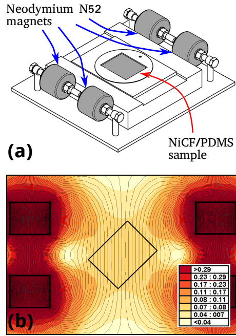
Figure 1: (a) Magnetic setup for specimen curing. The specimen is suspended in the centre of four Neodymium N52 magnets to produce a homogeneous magnetic field. (b) The magnetic field intensity calculated in the FE environment FEMM [26] for a specimen at 45^\circ . Note that the specimen is much thinner than the radius of the magnets, meaning the change in magnetic field through the thickness is negligible as confirmed by the even fibre distribution in the specimen cross-section observed by optical microscopy.
