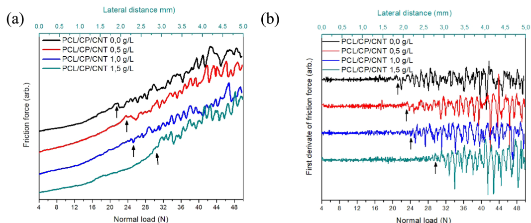
Figure 9. (a) Friction force and (b) first derivative of friction force versus normal load from 4 to 50 N of PCL/CP/CNT coatings with different concentration of multi-walled carbon nanotubes.
