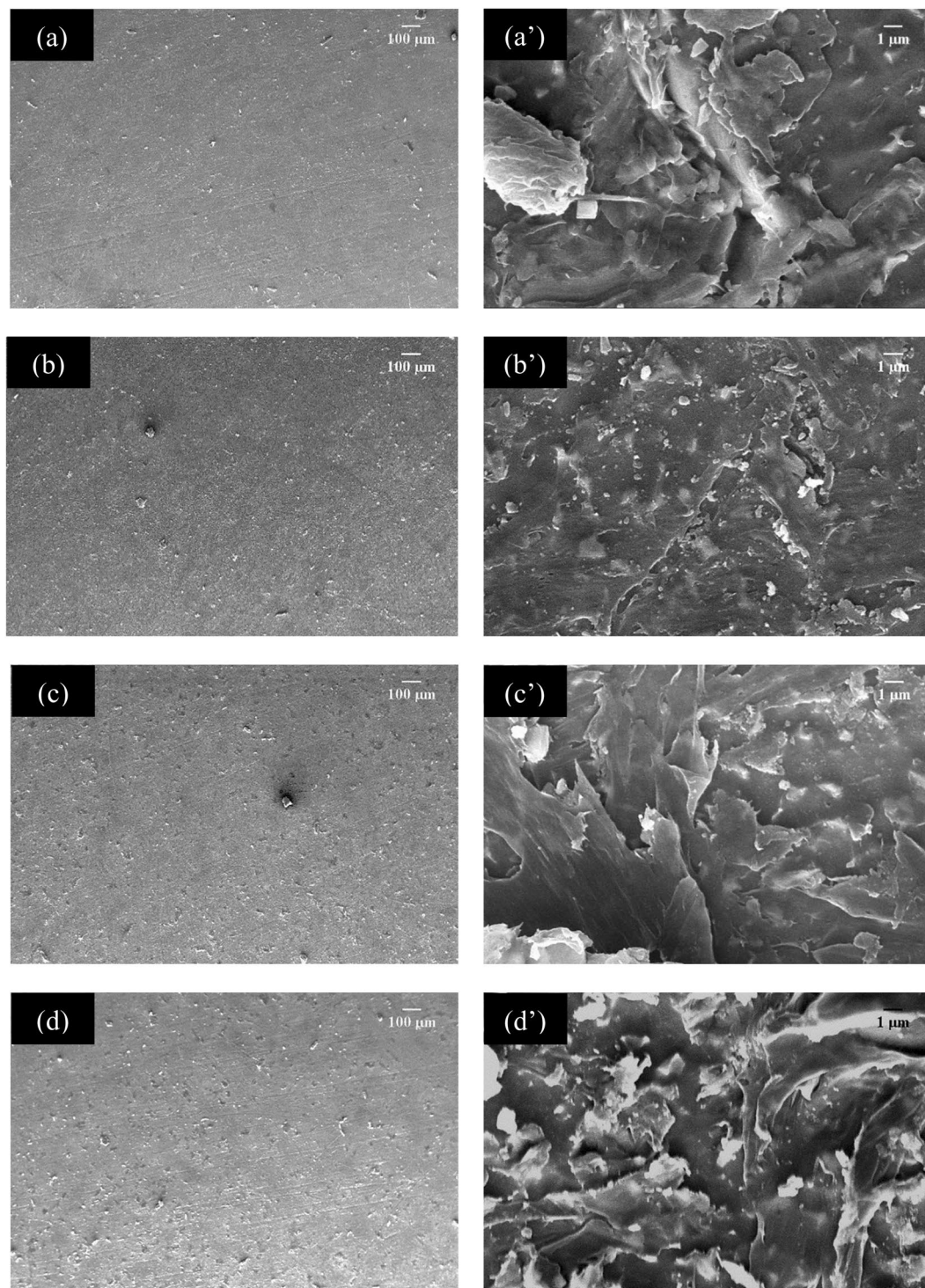
Figure 7. SEM micrographs of polycaprolactone-MWCNT/CP coatings (a,a') 0.0 g/L CNT, (b,b') 0.5 g/L CNT, (c,c') 1.0 g/L CNT and (d,d') 1.5 g/L CNT. The original magnification was 50X for (a–d) and 5000X for (a'–d'). Scale bar = 100 μm for (a–d) and scale bar = 1 μm for (a'–d').
