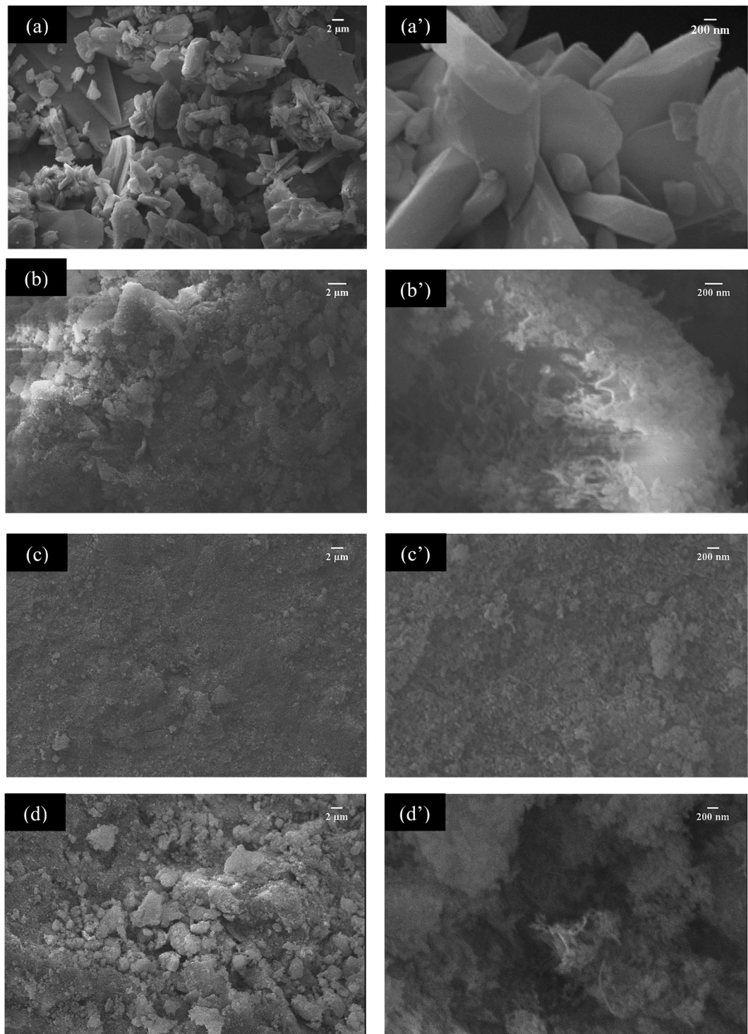
Figure 4. SEM micrographs of calcium phosphate and MWCNT powders ( a, a' ) 0.0 g/L CNT, ( b, b' ) 0.5 g/L CNT, ( c, c' ) 1.0 g/L CNT, and ( d, d' ) 1.5 g/L CNT. The original magnification was 2000X for ( a, c, d ) and 3000X for ( b ), 20000X for ( a', c', d' ) and 30000X for ( b' ). Scale bar = 2 \mu m for ( a–d ) and scale bar = 200 nm for ( a'–d' ). EDS spectrum can be seen in the inset in ( a–d ).
