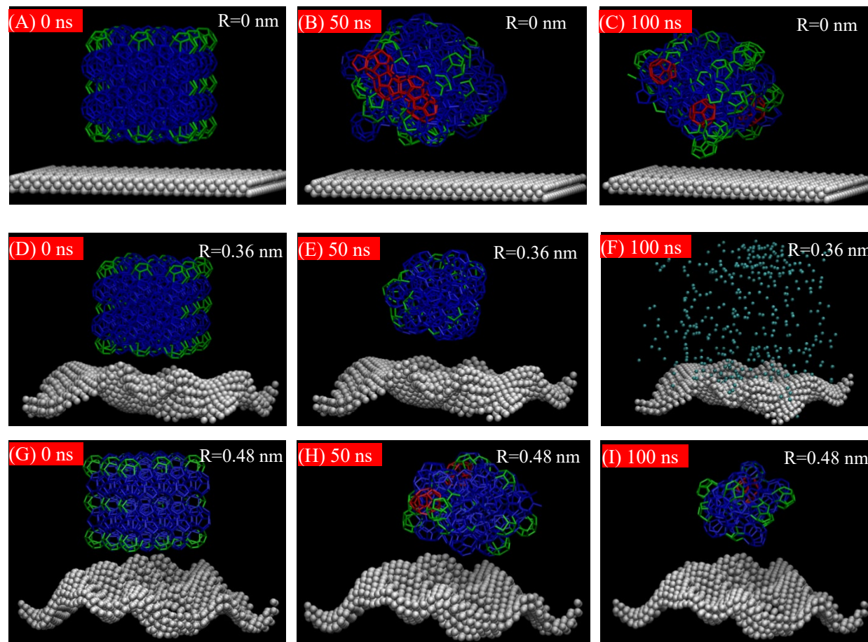
Fig. 1 Snapshots showing the evolution of methane hydrate clusters on solid surface with different roughness ( T=255 K, \varepsilon_{sw}=4.73 kJ mol -1 ). Solid surface: gray, 5^{12} cage: green, 5^{12}6^2 cage: blue, 5^{12}6^3 cage: red. Dispersed methane molecules (cyan balls) are only shown in panel F. The free water molecules are hidden in order to show the configurations of water cages more clearly.
