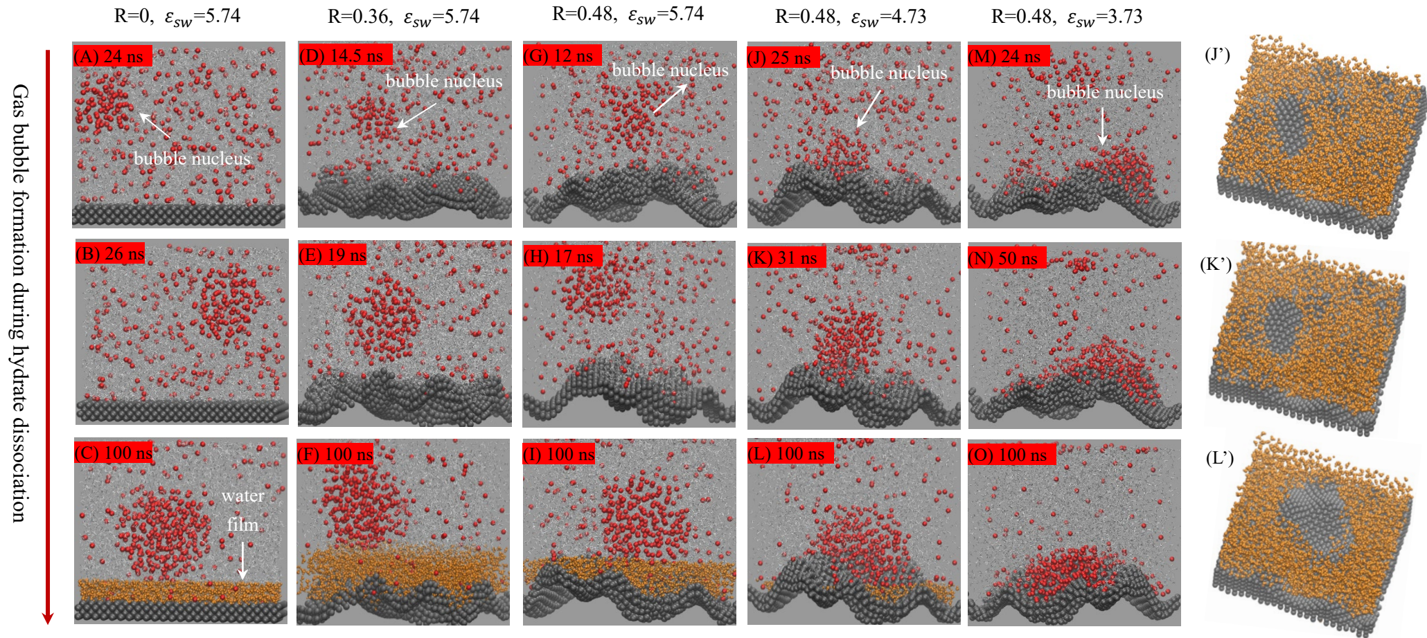
Fig. 6 Gas bubble evolution during hydrate dissociation on solid surfaces with various roughness ( R : nm) and hydrophobicity ( \epsilon_{sw} : kJ mol -1 ) at 260 K. Panel J'-L' is the vertical view of the water molecules below the gas bubble corresponding to J-L, respectively. Water film close to the substrate are highlighted in orange.
