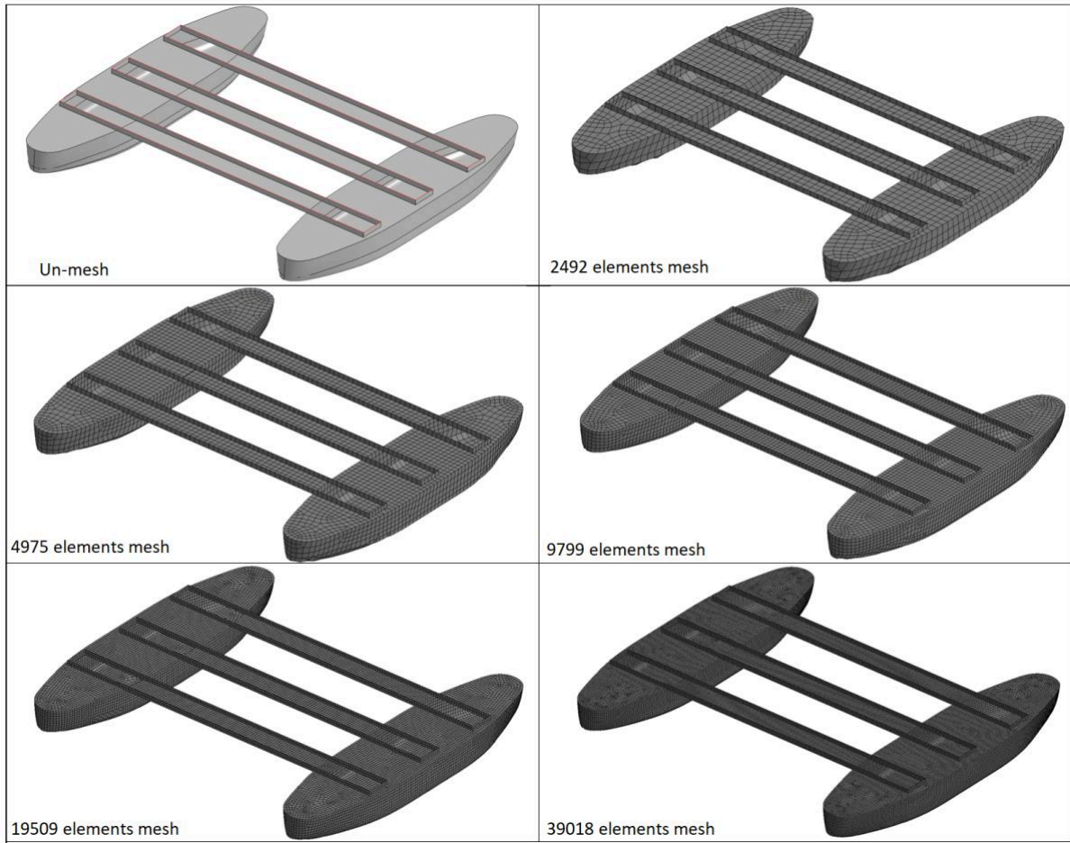
Figure 11. Progressive mesh sizes
