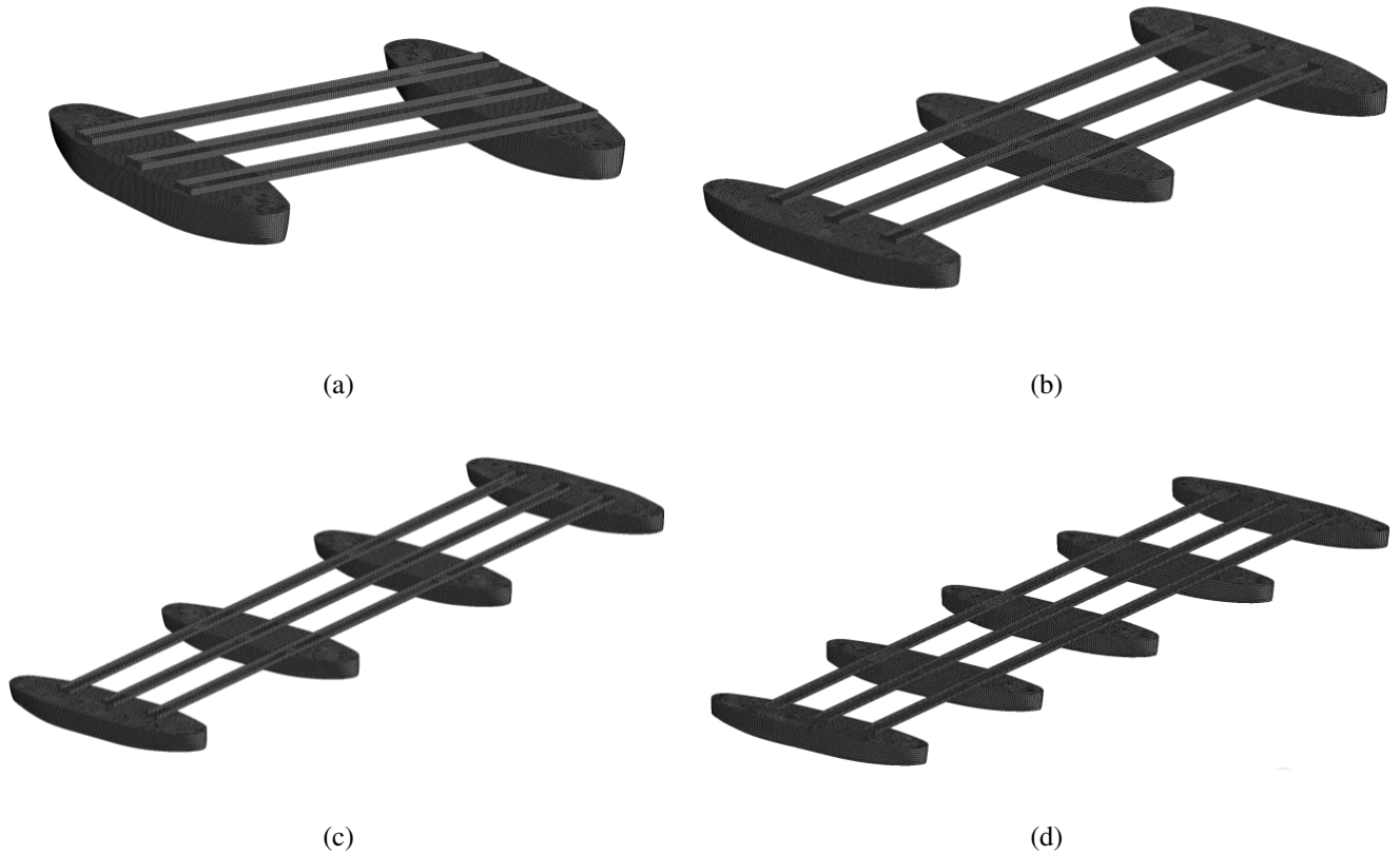
Figure 10. Mesh vizualization: (a) Catamaran, (b) Trimaran, (c) Quadrimaran, (d) Pentamaran
