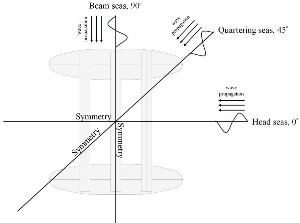
Figure 12. Wave heading
