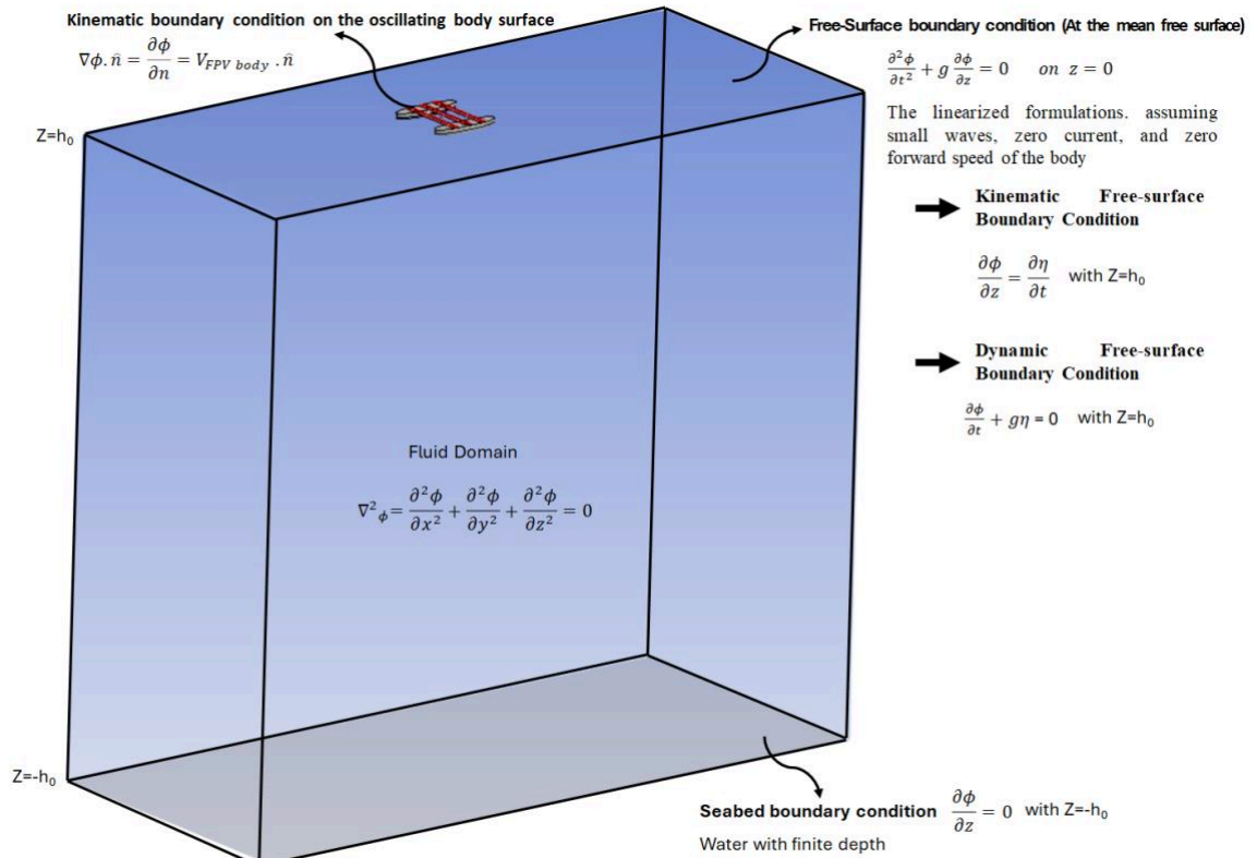
Figure 6. Boundary Condition
