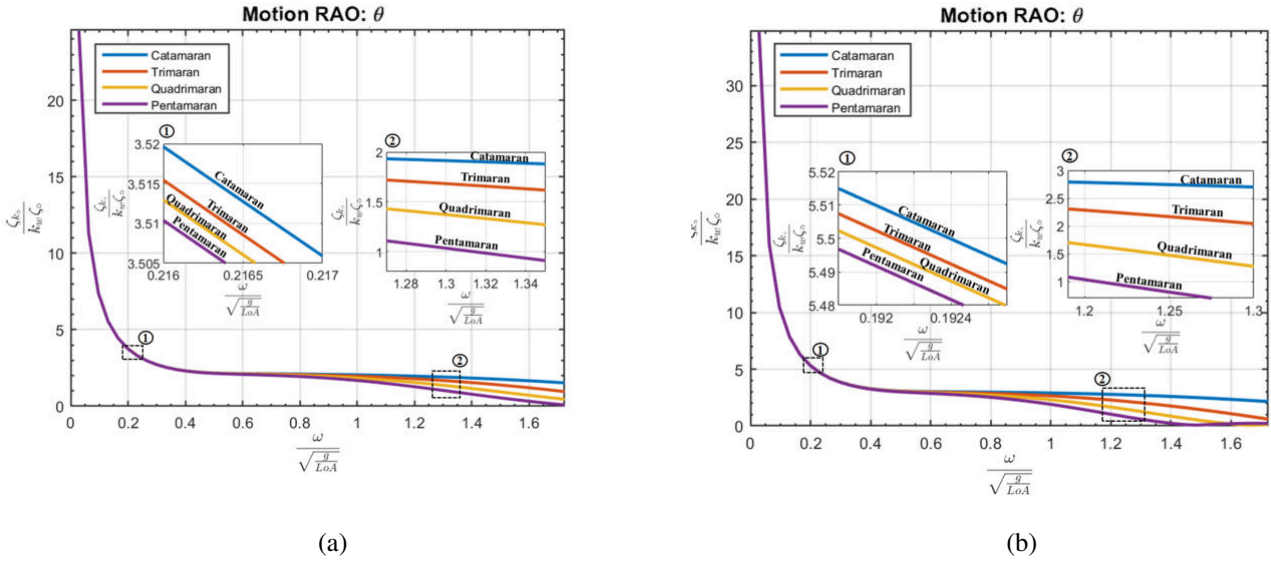
Figure 14. Global-RX ( \theta ) transfer function based on wave heading: (a) \varphi = 45^\circ , (b) \varphi = 90^\circ
