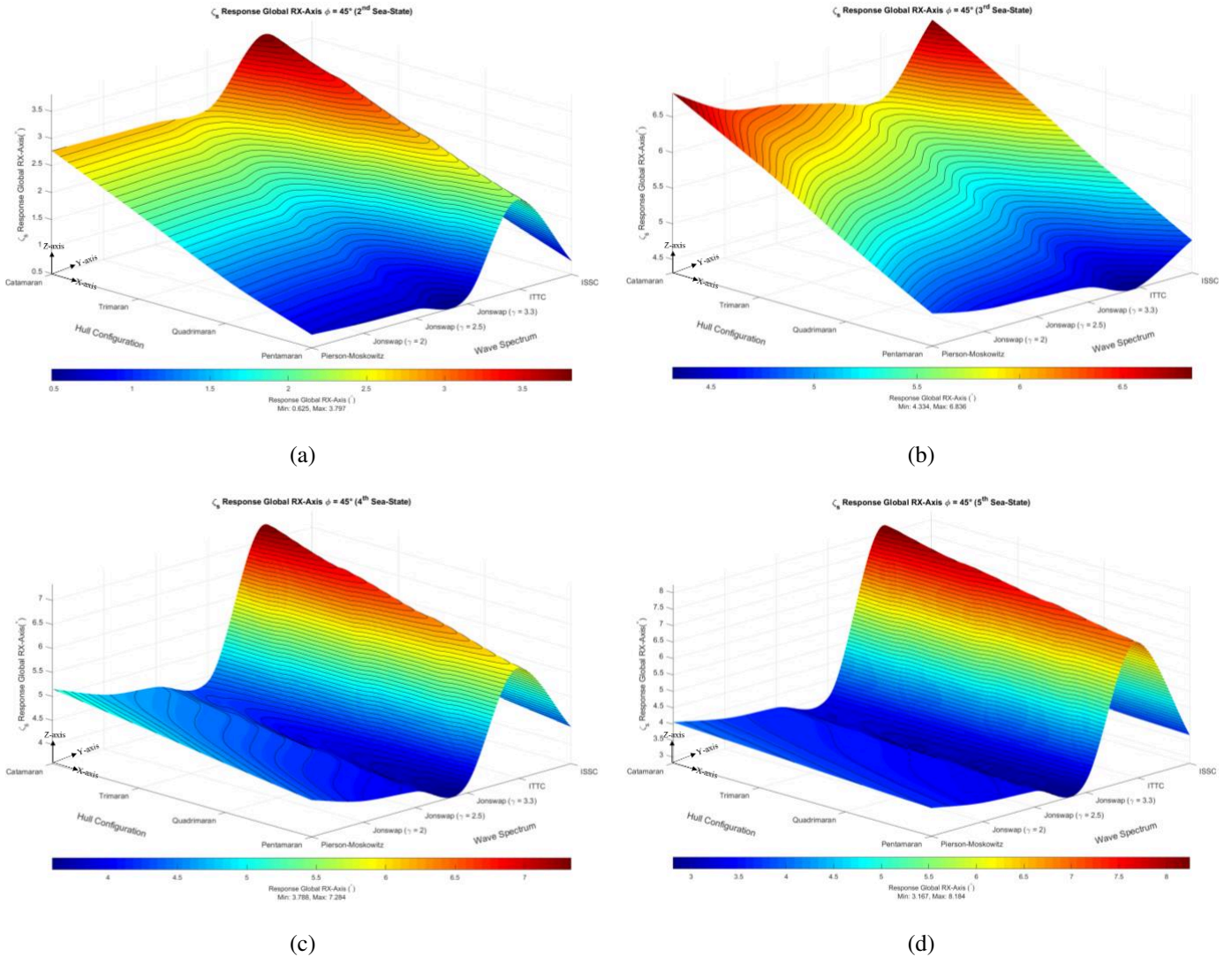
691 Figure 19. \zeta_s of roll in wave heading 45^\circ : (a) H_s = 0.50 m, (b) H_s = 1.25 m, (c) H_s = 2.50 m, (d) H_s = 4.00 m
