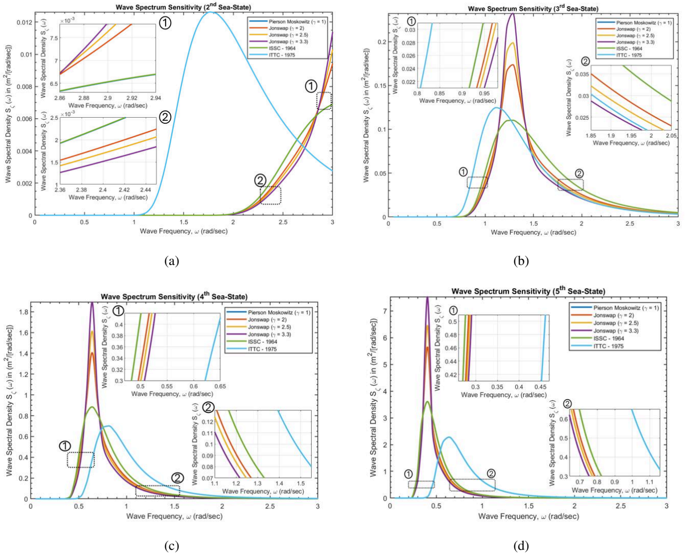
Figure 16. Irregular wave spectrum: (a) H_s = 0.50 m, (b) H_s = 1.25 m, (c) H_s = 2.50 m, (d) H_s = 4.00 m
