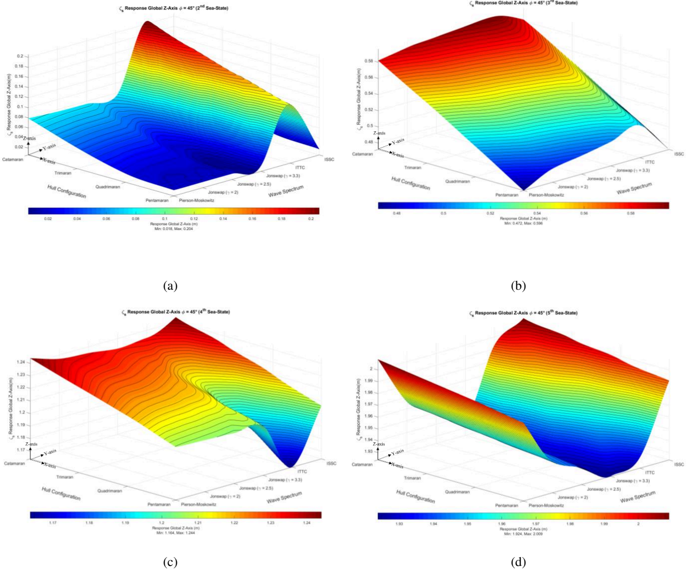
Figure 17. \zeta_s of heave in wave heading 45^\circ : (a) H_s = 0.50 m, (b) H_s = 1.25 m, (c) H_s = 2.50 m, (d) H_s = 4.00 m
