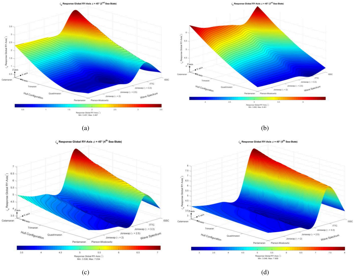
729 Figure 21. \zeta_s of pitch in wave heading 45^\circ : (a) H_s = 0.50 m, (b) H_s = 1.25 m, (c) H_s = 2.50 m, (d) H_s = 4.00 m
