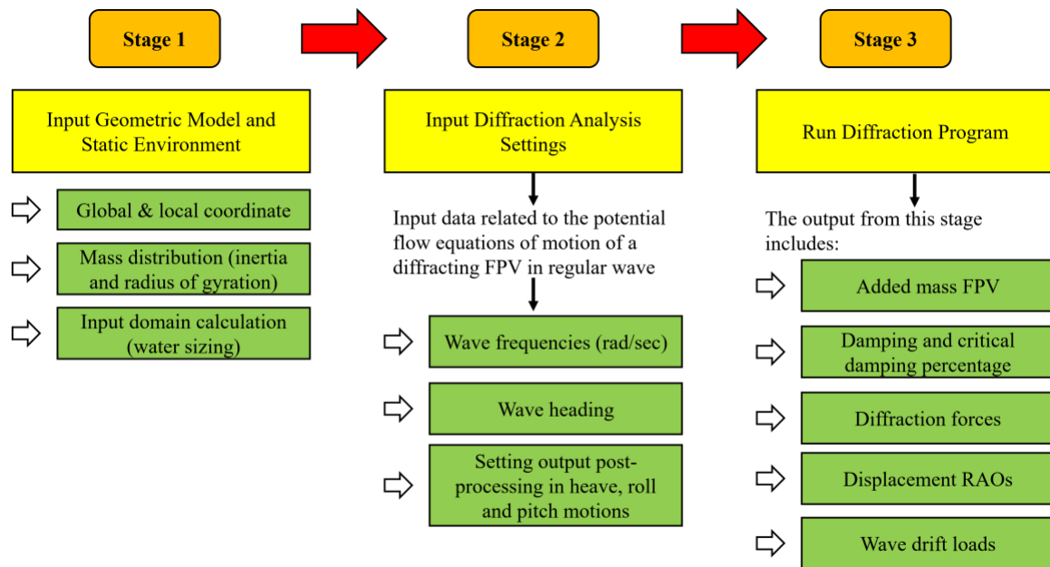
Figure 7. Stages of AQWA numerical analysis, redrawn from (Ansys, 2012)
