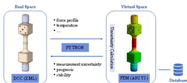
Figure 2. Developed concept of Digital Metrological Twin.
