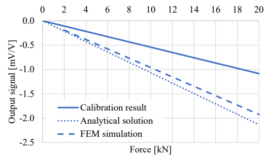
Figure 4. Simulated and experimentally measured output signal.
