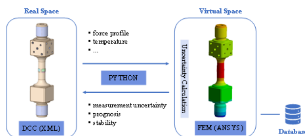
Figure 2. Developed concept of Digital Metrological Twin.
