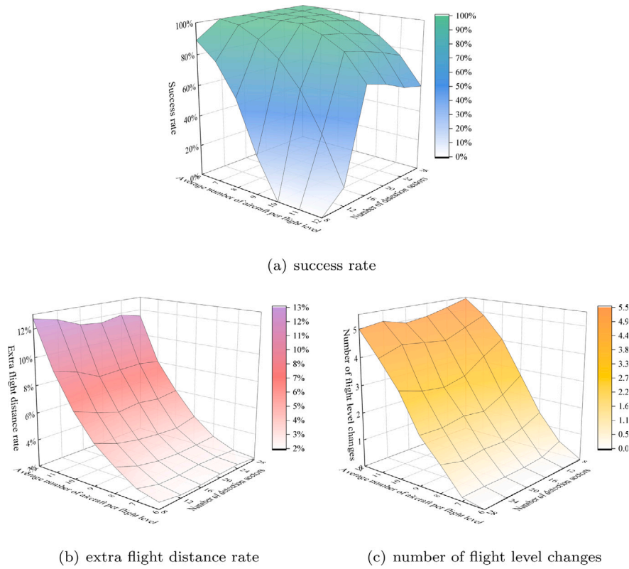
Fig. 17. Sensitivity analysis for number of detection sectors. Note that the orientation of the bottom axes (representing the average number of aircraft per flight level and/or detection range) in the three sub-figures may differ to facilitate the observation of trend changes.
