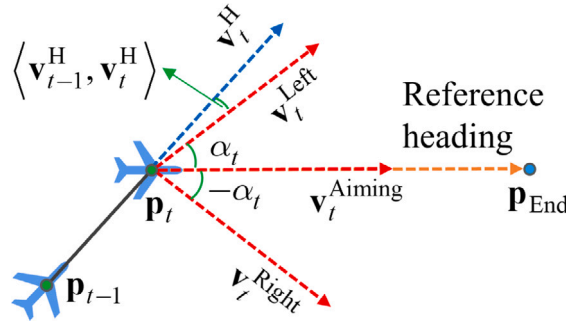
Fig. 3. Heading manoeuvre based on the agent's action. For example, if the agent intends to yaw to the left, its target heading v_t^H would be v_t^{Left} . Suppose the heading at the last time step is v_{t-1}^H . The turning angle for the current time step can be calculated as \langle v_{t-1}^H, v_t^H \rangle .
