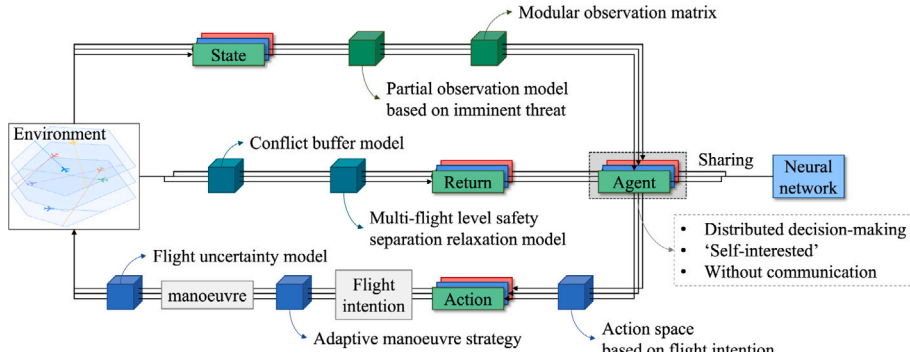
Fig. 2. Top-level framework of the MARL-based 3DMACR method.
