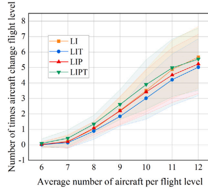
(c) number of flight level changes
