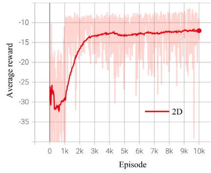
Fig. 18. Training results of the 2D model. The figure was generated using the Python toolkit for machine learning data visualisation, TensorboardX . The light curves represent the actual result data, while the dark curves are fitted based on the former, with a 95% smoothing coefficient to improve legibility.
