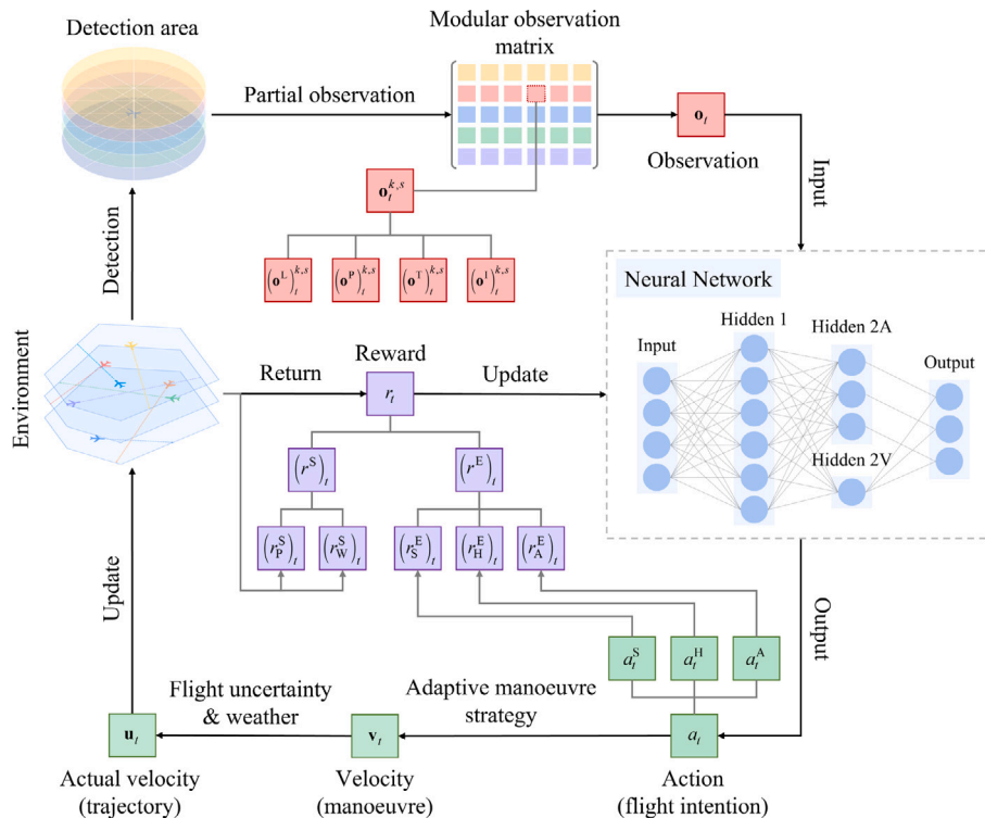
Fig. 9. Workflow of a single agent, which is part of Fig. 2. The neural network architecture is highlighted. The aircraft number i is omitted for clarity.
