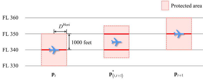
Fig. 7. Diagram of the multi-flight level safety separation relaxation model (2D side view). The protected areas are highlighted in red, but the dotted lines are not included. The thick red solid lines represent the flight levels and the corresponding ranges occupied by the aircraft.
