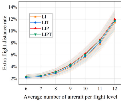
(b) extra flight distance rate
