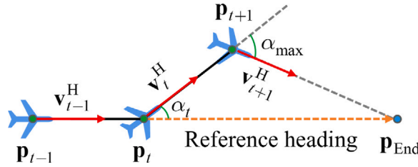
Fig. 4. Adaptive yaw angle. The yaw angle \alpha_t is adaptive to guarantee that the subsequent yaw angle meets the aircraft performance constraints.
