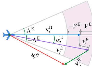
Fig. 5. Symbol schematic for the flight uncertainty model. The aircraft's horizontal velocity \mathbf{v}_t^H (blue arrow), error-based velocity \mathbf{v}_t^E (purple arrow), wind velocity \mathbf{v}_t^W (green arrow) and actual horizontal velocity \mathbf{u}_t^H (red arrow) are highlighted. The light purple area represents the range of error-based velocity \mathbf{v}_t^E .
