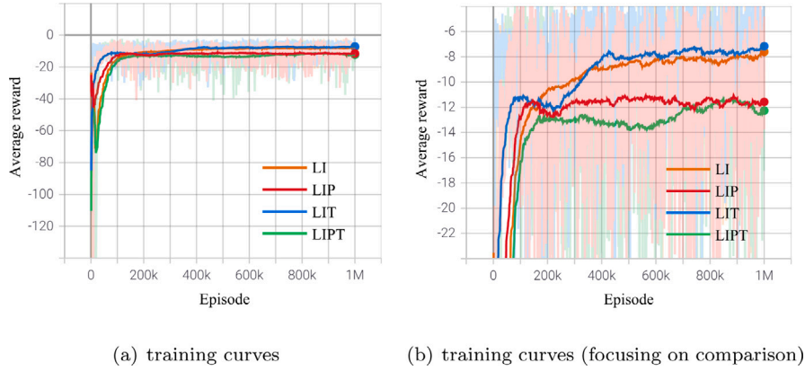
Fig. 12. Training results. The figure was generated using the Python toolkit for machine learning data visualisation, TensorboardX . The light curves represent the actual result data, while the dark curves are fitted based on the former, with a 95% smoothing coefficient to improve legibility. Sub-figure (b) is a zoomed-in version of sub-figure (a), focusing on the comparison of the four models. It shows the average reward in the range of -22 to -6 .
