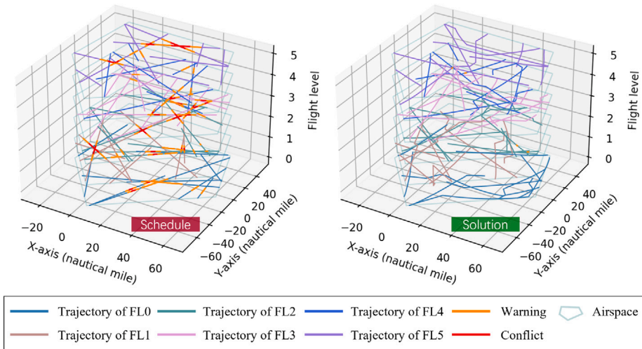
Fig. 14. Comparison of trajectories before and after conflict resolution (global view).
