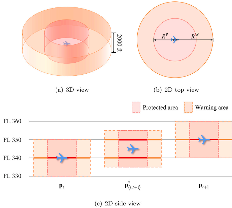
Fig. 8. Diagram of the conflict buffer model.
