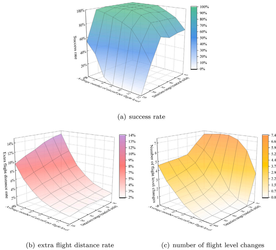
Fig. 16. Sensitivity analysis for detection range. Note that the orientation of the bottom axes (representing the average number of aircraft per flight level and/or detection range) in the three sub-figures may differ to facilitate the observation of trend changes.
