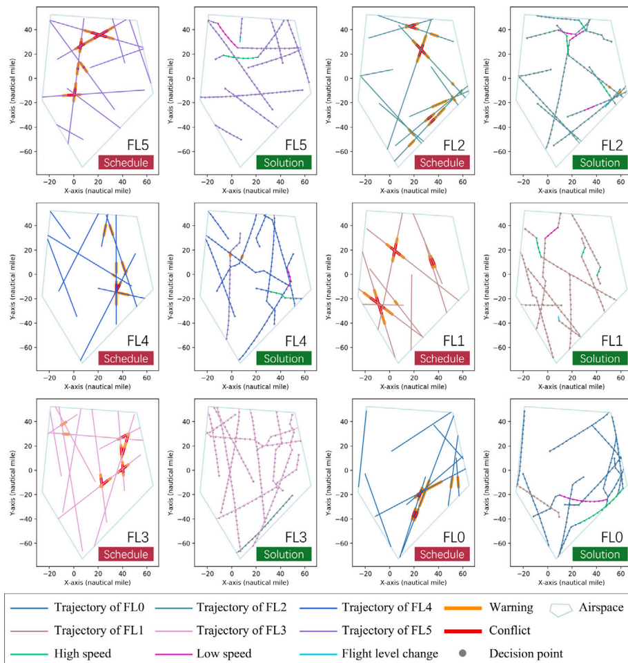
Fig. 15. Comparison of trajectories before and after conflict resolution (flight-level view). This figure is generated using the data from the same case as Fig. 14.
