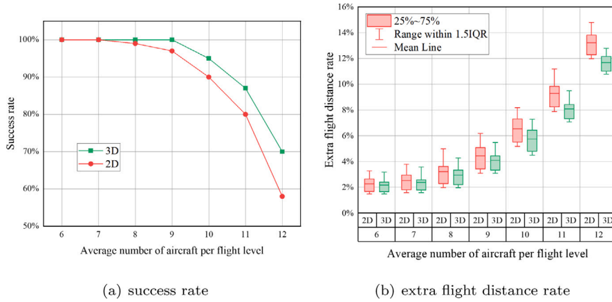
Fig. 19. Performance test results for 2D and 3D models.
