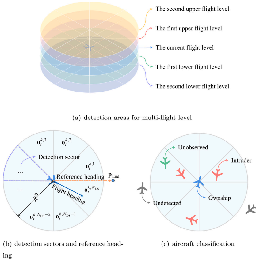
Fig. 6. Partial observation based on imminent threats for multi-flight level.
