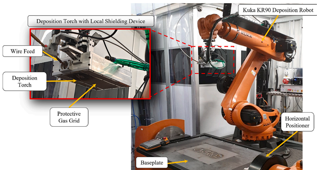
Fig. 2. WAAM deposition robot featuring a plasma arc process.
