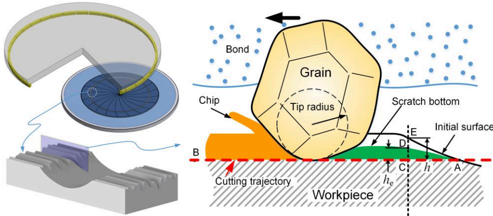
Fig. 3. A schematic illustration of scratch trajectory at a given instance chosen randomly on the inclined surface showing the cross-sectional view.
