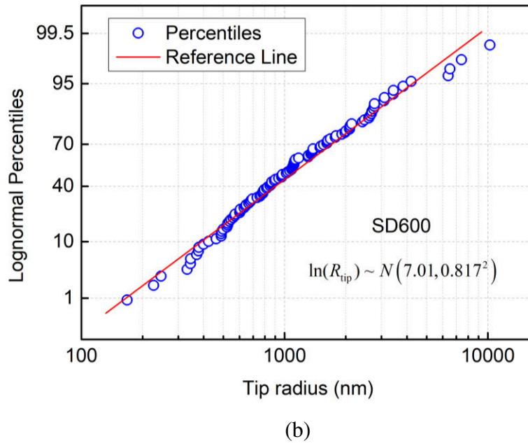
Fig. 8. Lognormal probability plot of the grit tip radius of wheel SD3000 (a) and SD600 (b). The experimental data set (scatter) is plotted against a theoretical lognormal distribution set (red line). The scatter points are close to the theoretical line which indicates that the grit tip radius can be well described by the lognormal distribution.
