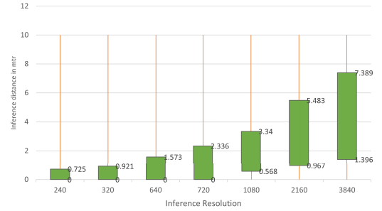
Figure 9. Inference distance for YOLOv8n with RAdam Optimiser
