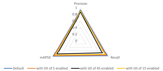
Figure 7. Precision-recall-mAP comparison of Nano models for different tilt angles
