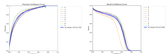
Figure 11. Precision-Confidence curve and Recall-Confidence curve for YOLOv8 with compound tuning
