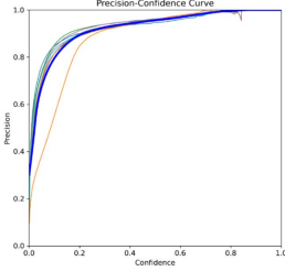
Figure 4. Precision-Confidence Curve of YOLOv8x, YOLOv8n, YOLOv8m
