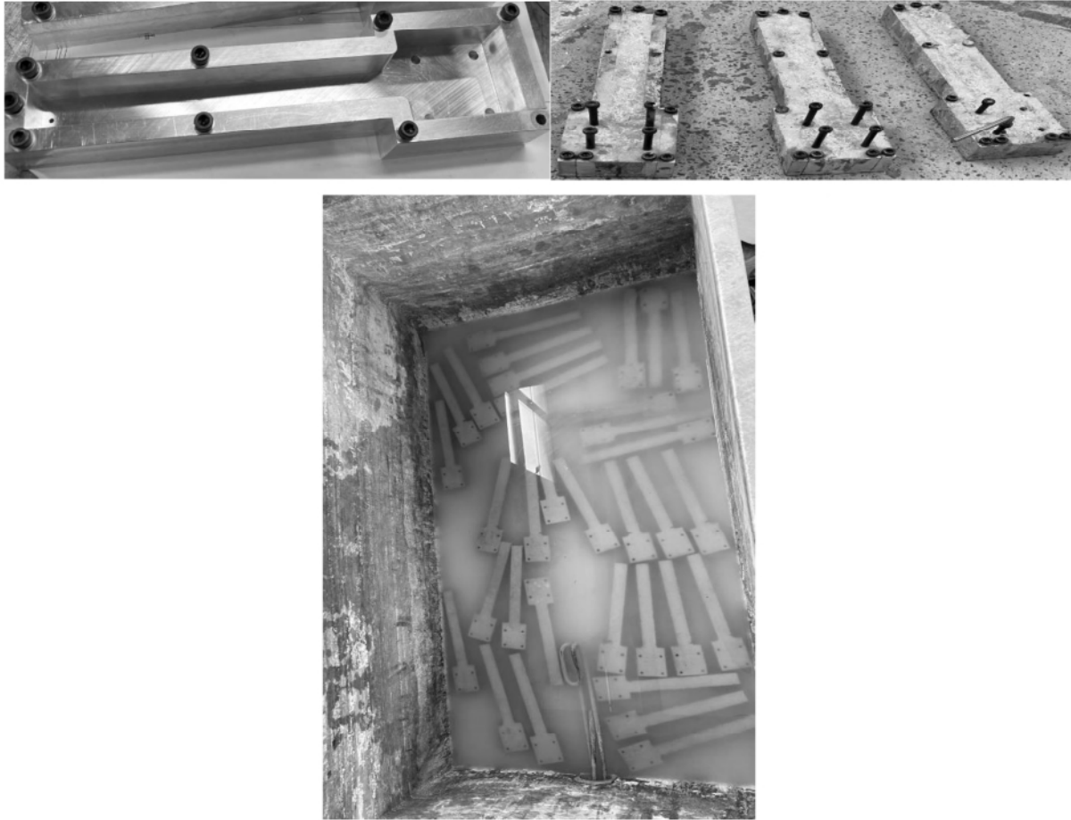
Figure-2 Beam sample preparation.
