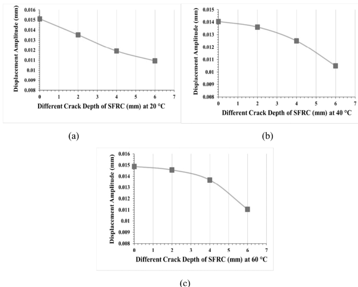
Figure-11 Displacement amplitudes of SFRC measured experimentally at various crack depths and temperatures.
