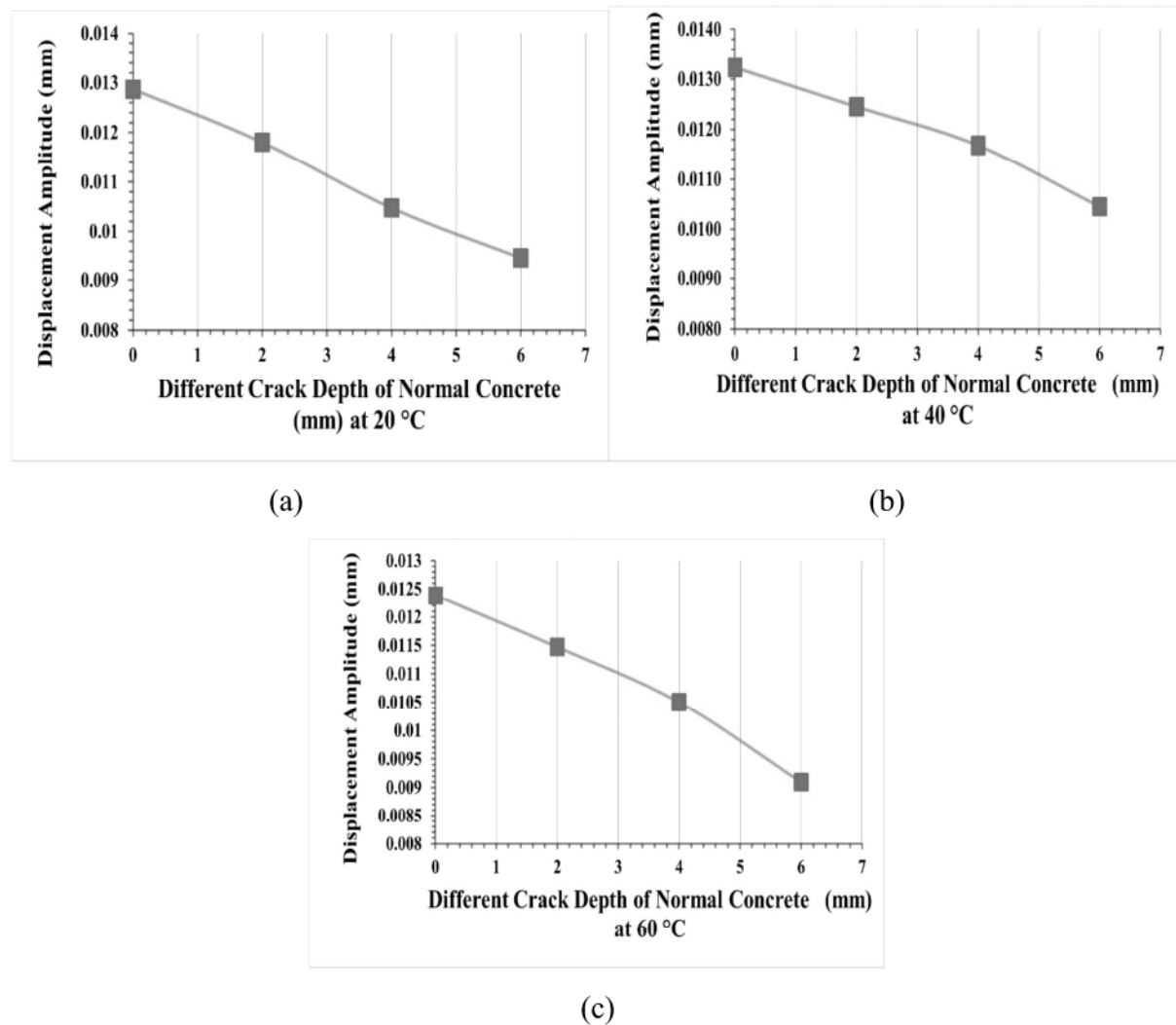
Figure-10 Displacement amplitudes of normal concrete measured experimentally at various crack depths and temperatures.
