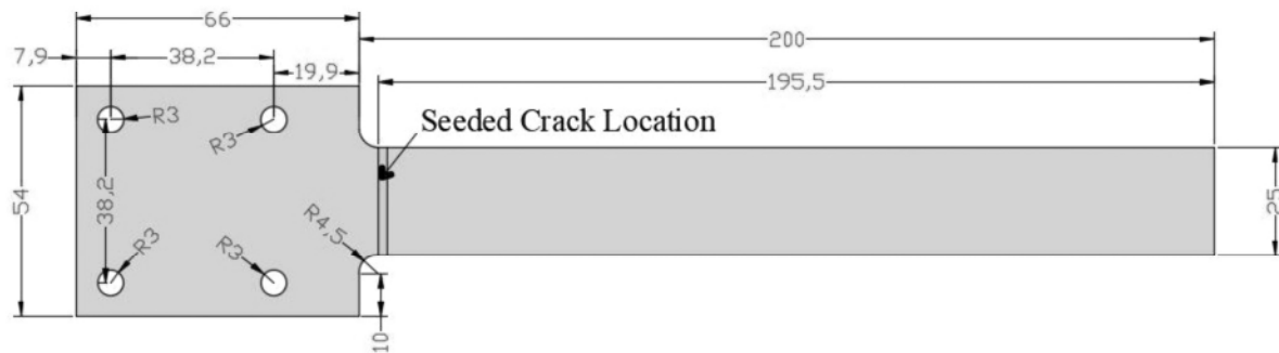
Figure-1 Geometry of a beam with dimensions of 200 mm, 30 mm, and 25 mm.
