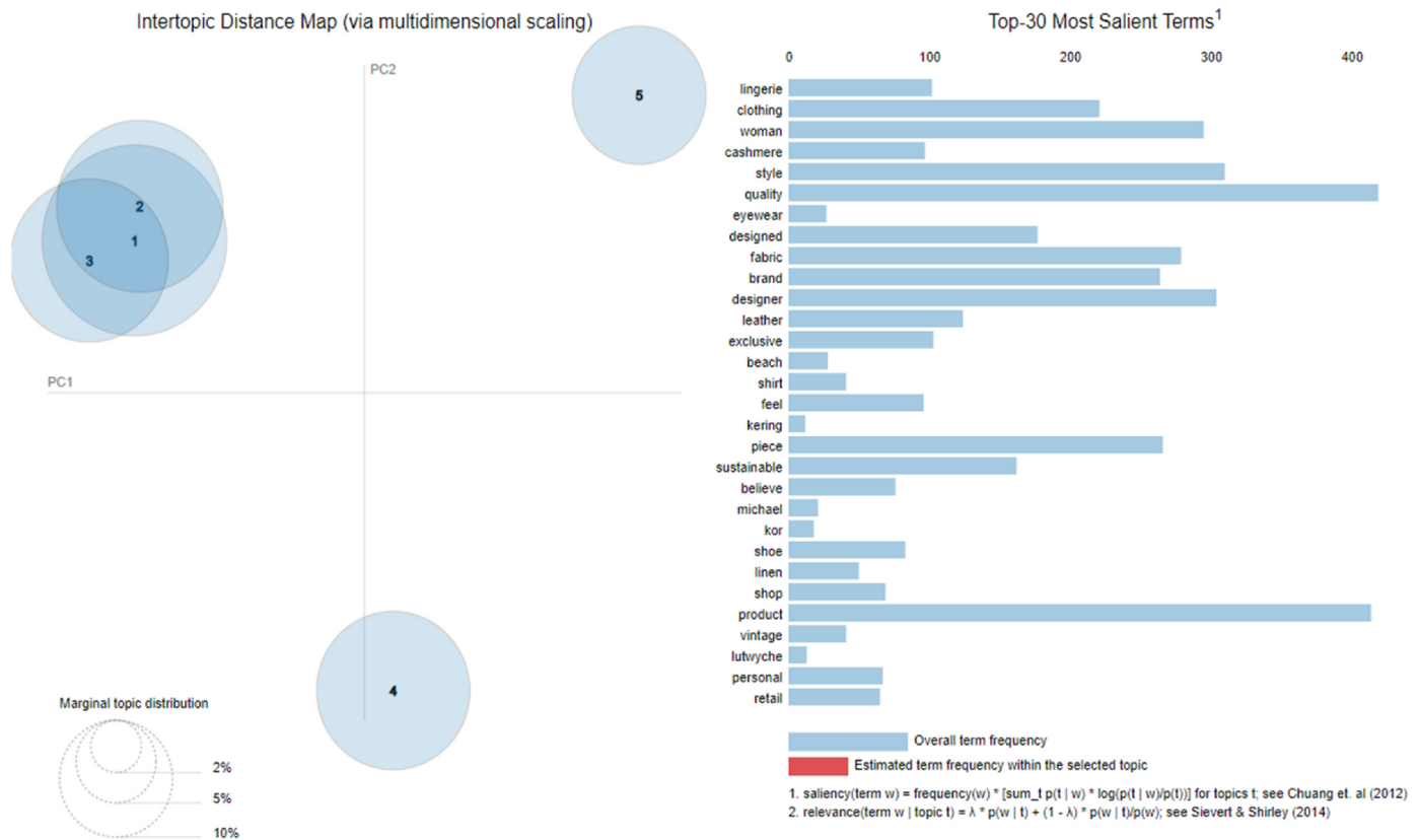
Fig. 4. LDA 5-topic configuration visualising the intertopic distances and most salient words for the analysed text corpus.
