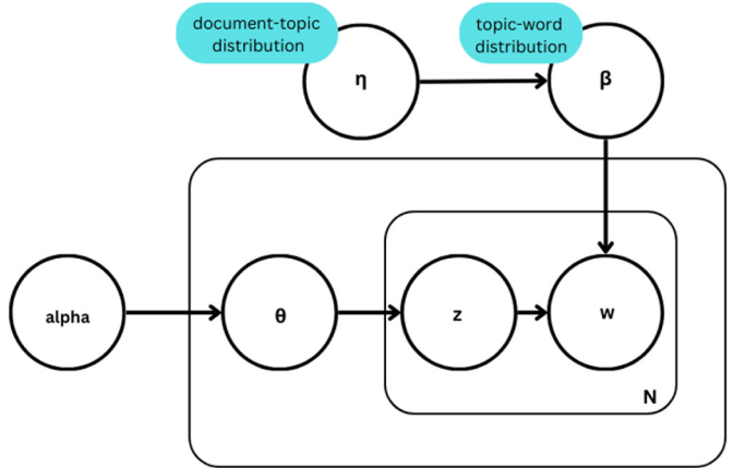
Fig. 3. LDA model architecture including the key parameters affecting the model’s performance.
