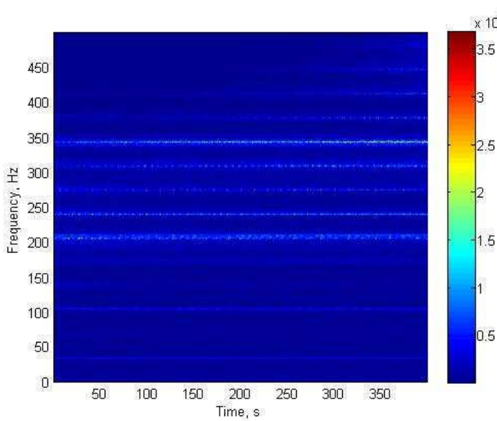
Figure 5: Spectrogram of static unbalanced rotor rotating at 35 Hz
