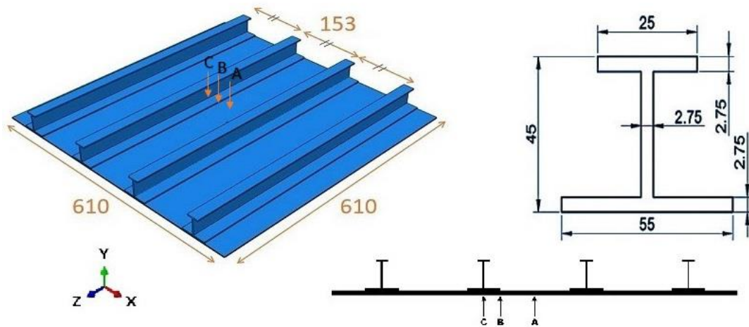
Figure 1. Panel Geometry and Impact Positions A, B &amp; C
