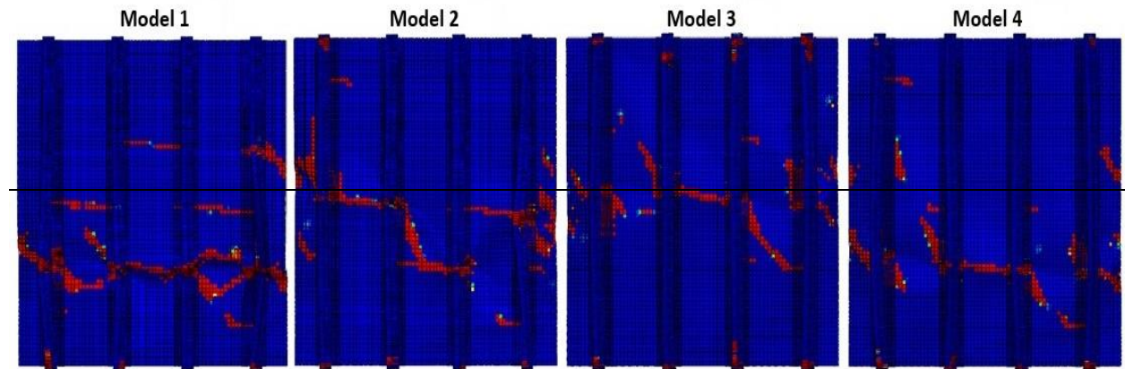
Figure 2. Matrix Compression Damage in the four initial models
