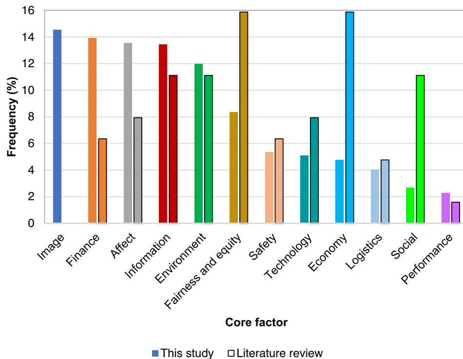
Fig. 14. Comparison between core factors of domestic hydrogen acceptance identified in this study and literature review.
