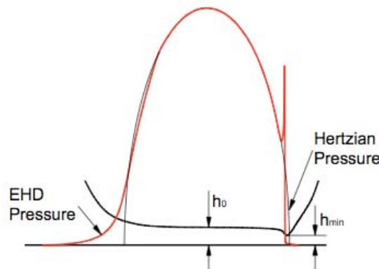
Figure 8: Elastohydrodynamic conjunction
