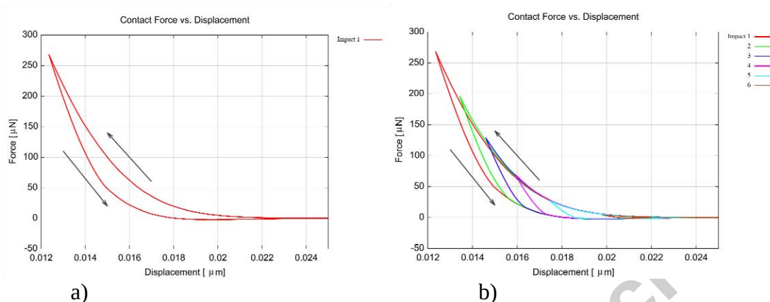
Figure 13: Impact and rebound in a nano-scale conjunction
